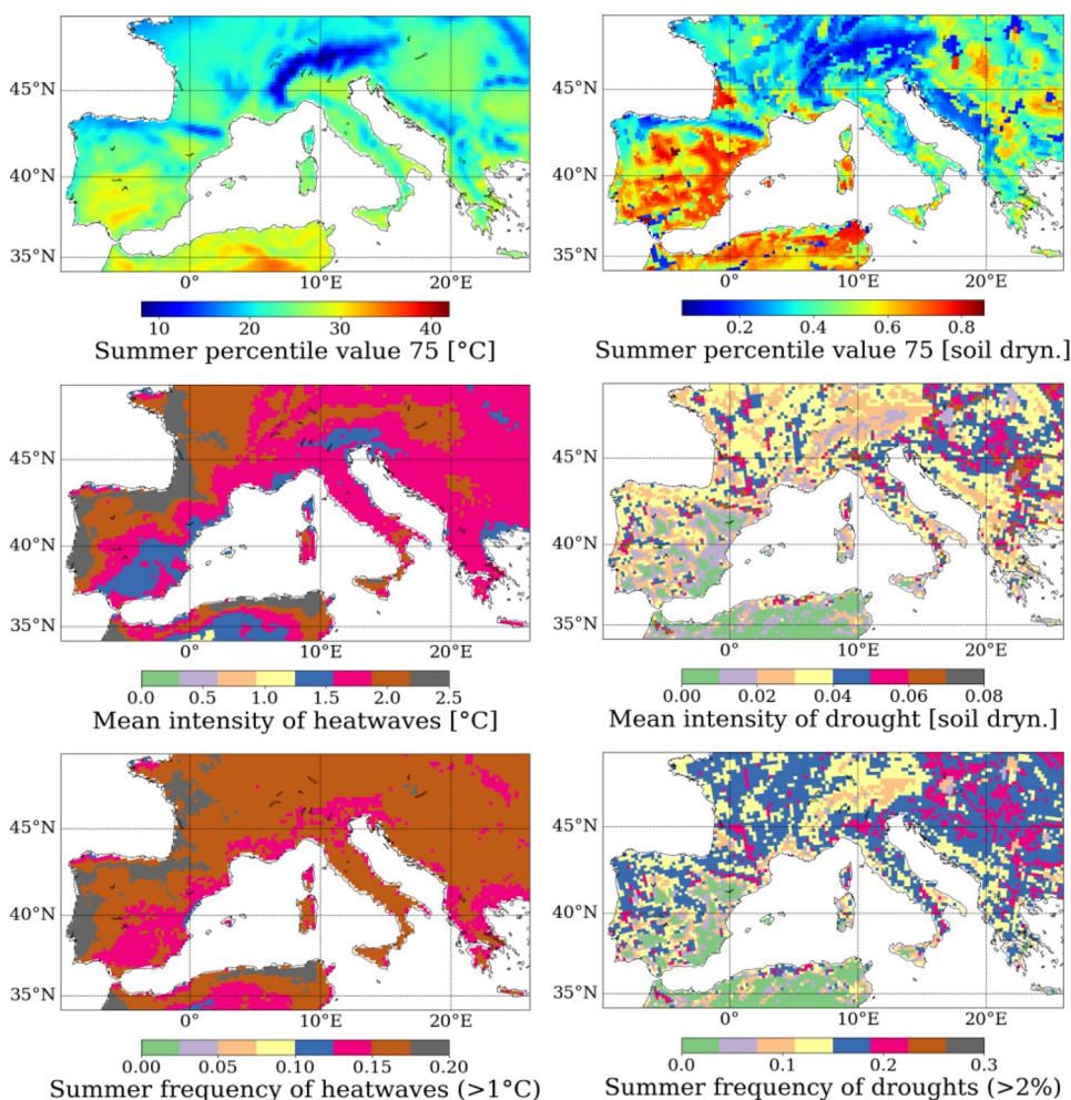
Fig. 4 Heatwaves (left column) and droughts (right column) identified using the Percentile Limit Anomalies (PLA) method. The first row shows the 75th percentile value during summer (JJA average), the second row shows the mean intensity of the extreme events, and the last row shows the frequency (over the total number of summer days) of intense events ( > 1\text{ }^{\circ}\text{C} for heatwaves and > 0.02 of soil dryness for droughts)
