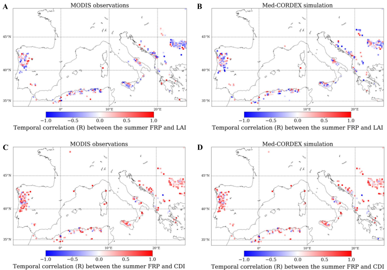
Fig. 11 Spatial distribution of temporal correlation (R) between summer Fire Radiative Power (FRP) and Leaf Area Index (LAI) from MODIS (A) and from Med-CORDEX (B) for areas of high fire activity (pixels with at least 1 km 2 of burned area for minimum 3 summers over 2003–2016). Same criteria of correlation are applied
