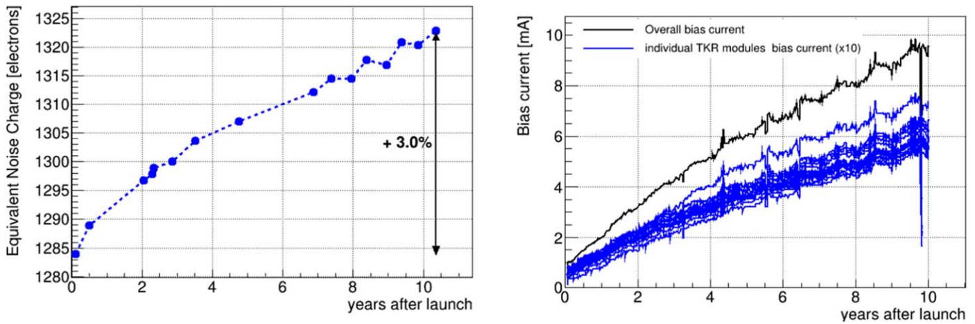
Figure 12. Left: tracker equivalent noise charge (ENC) trending (average over all strips; statistical error bars are smaller than markers dimension). Right: tracker bias current trending.
