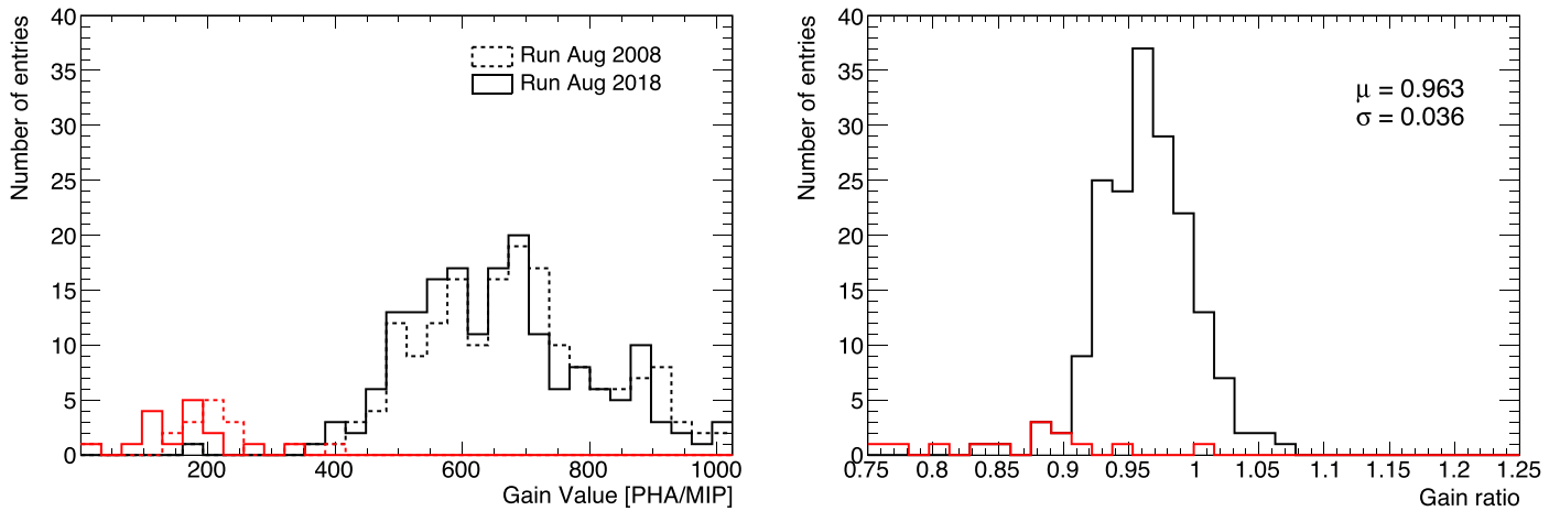
Figure 24. Comparison of the ACD channel gains for a reference run in the early mission with a run 10 yr into the mission (left) and the gain ratios for the two runs (right). Channels associated with ACD tiles are shown in black while channels associated with ACD ribbons are shown in red.
