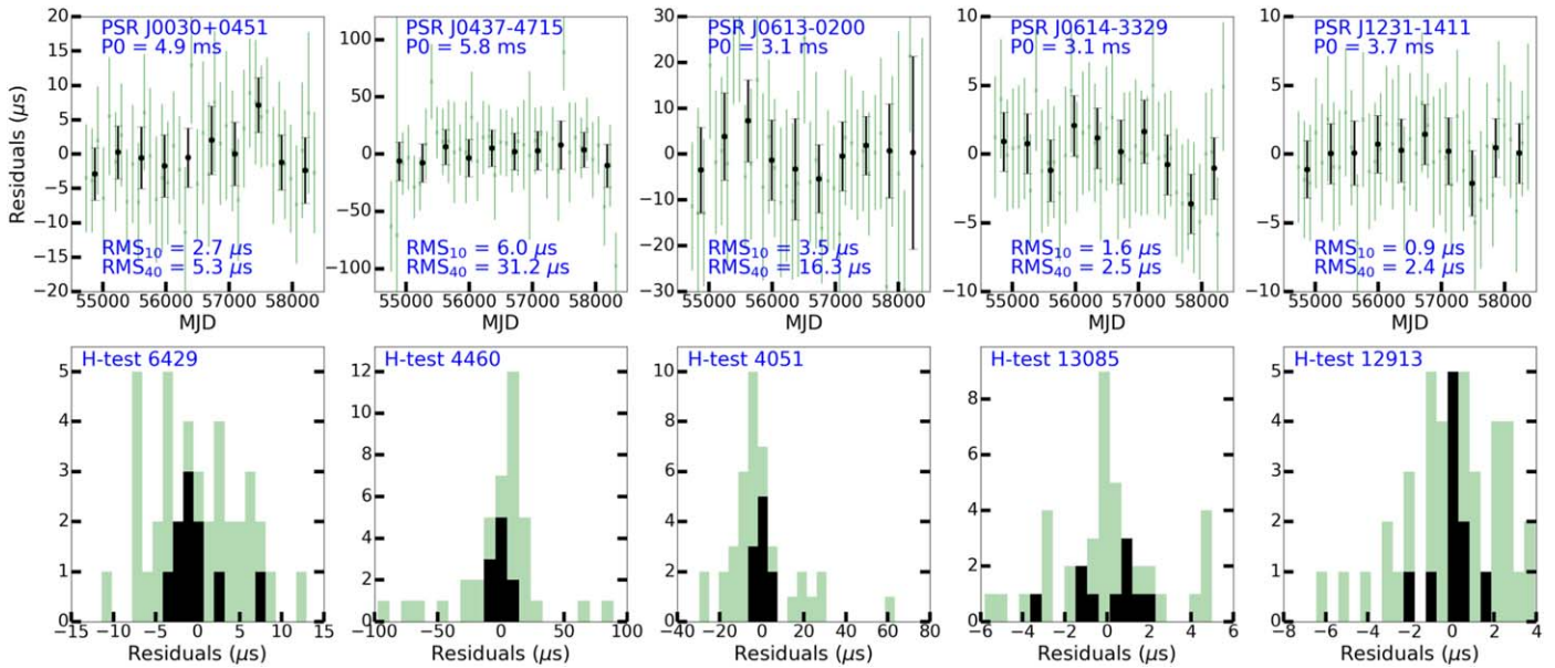
Figure 25. Stability of gamma-ray millisecond pulse times compared to radio references. Top: black dots show ten one-year average values, and green crosses show 40 three-month average values. The rms variations are dominated by the statistical uncertainties in both the gamma-ray and radio data. Bottom: the same points, displayed as histograms. The H-test indicates the statistical significance of the pulsed signal (see text).
