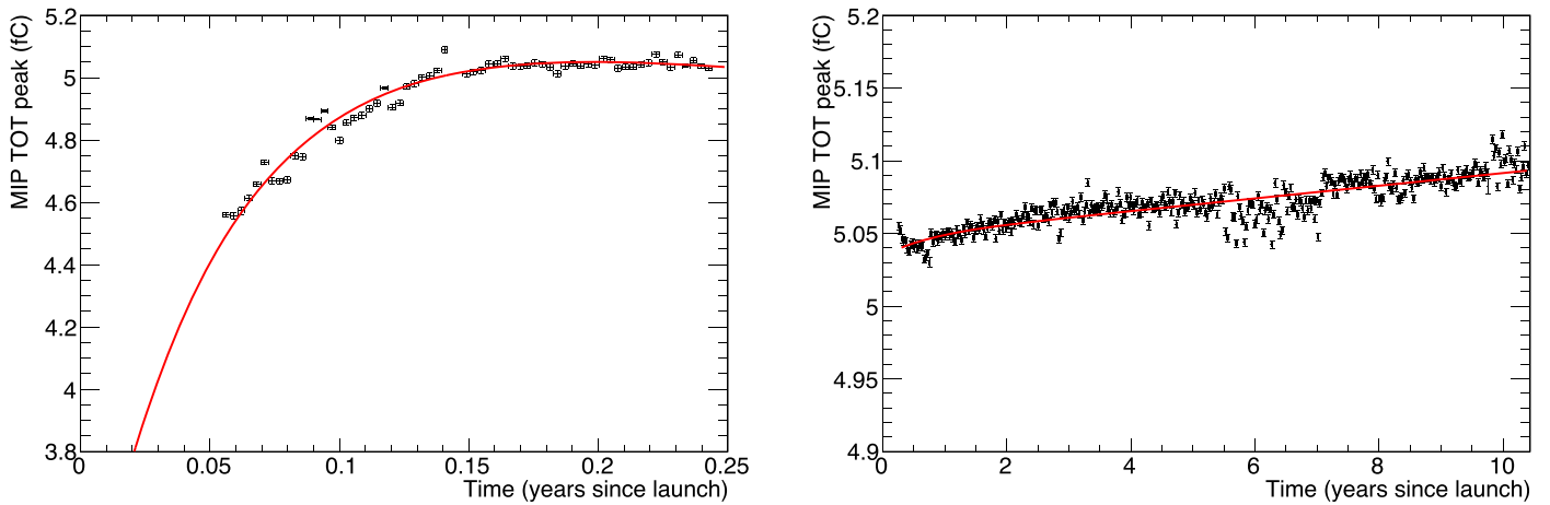
Figure 9. Trending of the minimum ionizing particle (MIP) peak energy value during the first weeks after launch (left) and for the remainder of the mission (right).
