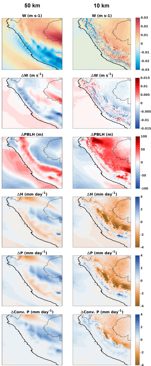
Fig. 9 Annual mean vertical velocity at ~500 hPa ( W in \text{m s}^{-1} ) and projected changes in vertical velocity ( \Delta W ), planetary boundary layer height ( \Delta\text{PBLH} in m), dry static energy flux divergence ( \Delta H in \text{mm day}^{-1} ; see Eq. 1), total precipitation ( \Delta P in \text{mm day}^{-1} ) and convective precipitation ( \Delta\text{Conv. P} in \text{mm day}^{-1} ) according to WRF results in 50 and 10 km horizontal resolution over Peru. Results are averaged over the three simulations WRF_CESM, WRF_CCSM4 and WRF_ACC and changes are between 1996–2005 and 2091–2100. Results for central Chile and southern Brazil are in Supplementary Fig. S11
