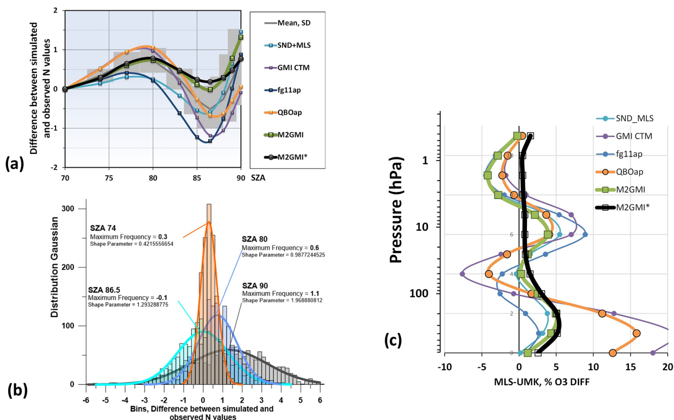
Figure 2. The simulated Umkehr observations are based on the GMI CTM and M2GMI models, MLS satellite overpass and ozonesonde profiles at Boulder, and two ozone climatologies at 40^\circ latitude (fg11ap and QBOap). (a) Difference between simulated and observed N values at Boulder as a function of SZA. (b) Histogram of the differences between simulated (based on M2GMI data) and observed N values at 74^\circ (orange), 80^\circ (purple), 86.5^\circ (light blue), and 90^\circ (dark) SZA. Solid lines are normal distribution fits to the data; the maximum frequency and shape parameters of the fit are provided in the legend. (c) The difference between the MLS and several versions of Umkehr profiles retrieved after applying corrections shown in panel (a). The final optimized adjustment M2GMI* ( N -value correction is shown in panel a as a black line) is found through the iterative approach to minimize the M2GMI bias.
