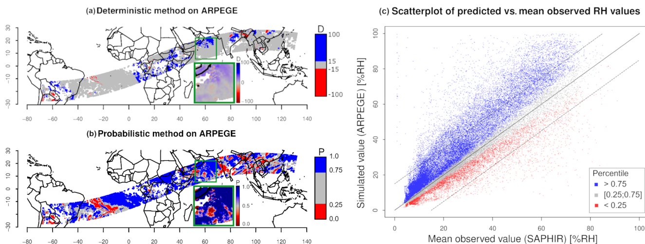
Figure 5. Comparisons between SAPHIR's \overline{RH_{obs}} and ARPEGE's RH_{mod} on 1 April 2018 at 00:00 UTC and for the 400–600 hPa atmospheric layer. (a) Map of the difference D , (b) map of the probability P , and (c) scatterplot between \overline{RH_{obs}} ( x axis) and RH_{mod} ( y axis); the percentile associated with each point is P > 0.75 (blue), 0.25 < P < 0.75 (gray) and P < 0.25 (red); the solid line represents the y = x line, and the dotted lines delimit the \bar{x} \pm 15\% RH around values.
