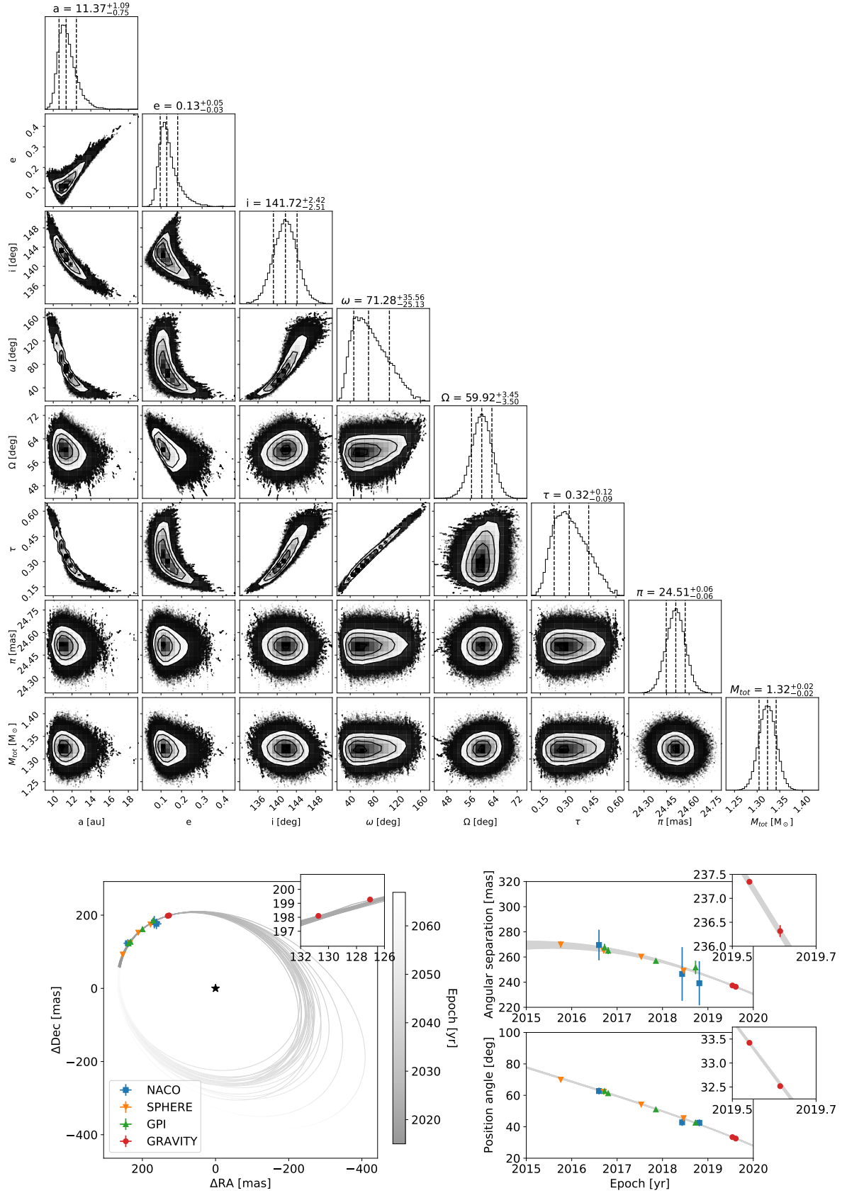
Fig. A.1. Same as Fig. 3, but using Gaussian priors of 140 \pm 3 deg for the inclination i and 61 \pm 4 deg for the longitude of the ascending node \Omega in order to enforce coplanarity between the orbit of HD 206893 B and the debris disk of the system.
