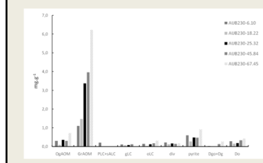
Fig. 8 Distribution of the different particles in the AUB230 borehole (6.10, 18.22, 25.32, 45.84, 67.45 m) and images of the particles encountered, scale 100 µm
