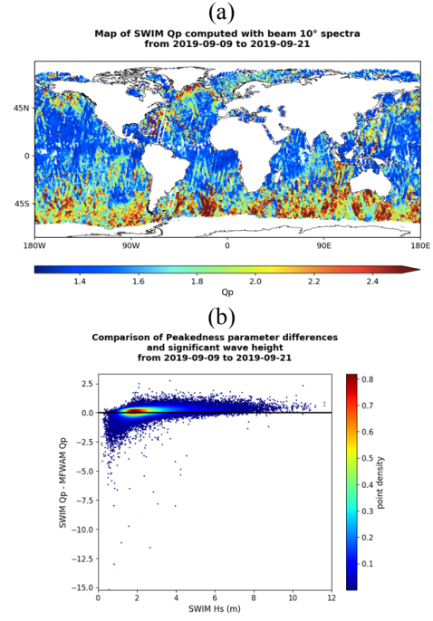
Fig.3 Same as in Fig.2 but for the parameter Q_p .
