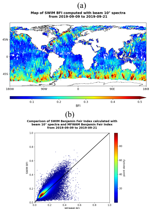
Fig.5 : (a) Map of BFI from SWIM (b) Histogram of BFI (SWIM versus MFWAM)
