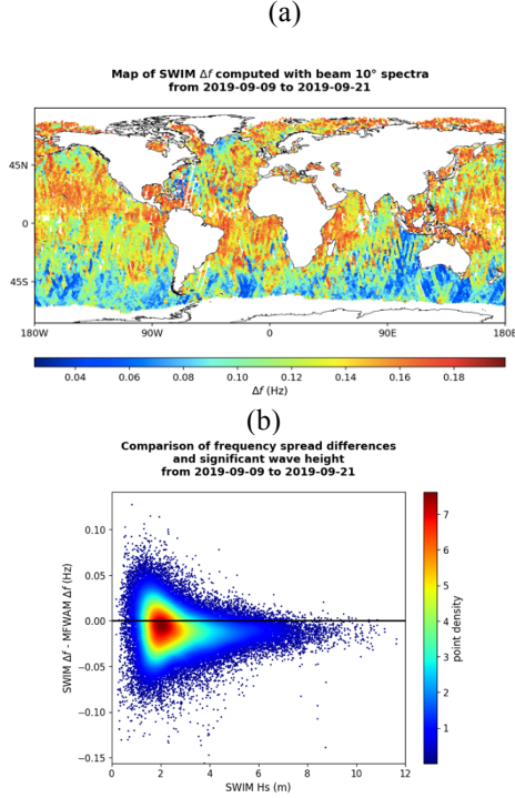
Fig.2 : (a) Map the parameter of spectral width \sigma_f deduced from the SWIM spectra. (b) histogram of the differences of \sigma_f values between SWIM and MFWAM as a function of the SWIM significant wave height. The data set is from 9 to 21 September 2019.
