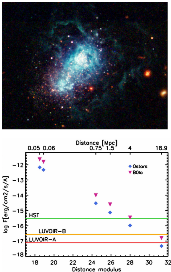
Fig. 10 Top: With a metal content of 1/32 Z_{\odot} , I Zw18 represents the next step down in the metallicity ladder towards the metal-free early Universe. I Zw18 has a demonstrated content of massive stars, but being \sim 18 Mpc away current facilities cannot resolve its stellar population. Bottom: Expected UV fluxes at 1500 \text{ \AA} for OB stars located at successively farther galaxies, compared to the performance of HST and the two LUVUOIR architectures. The stellar UV fluxes are typical values found in IC1613 scaled by distance. The plotted sensitivity of HST represents the faintest flux for which five orbits grant a spectrum with sufficient quality for quantitative analysis; this flux was scaled by mirror surface to estimate how deep LUVUOIR would reach. LUVUOIR-A will enable breakthrough spectroscopy of individual bright OB stars in I Zw18
