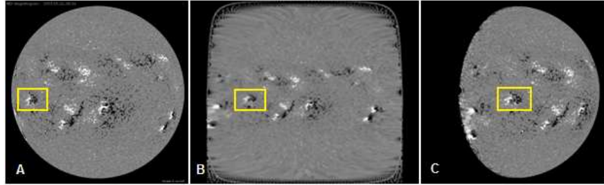
Figure 3. The three images above shows the re-mapping stages and how it affects an investigated region. Image date: 2003.05.22 06:24. Region NOAA number: 365. (A) The original magnetogram image in Heliocentric Cartesian coordinates. (B) The solar disk represented in Carrington Heliographic coordinates. (C) The solar disk re-mapped and represented in Heliocentric Cartesian coordinates, showing the active regions under investigation near the centre.
