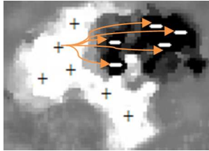
Figure 1. A sample of an active region showing the interaction between opposite polarity areas according to the magnetic complexity model. Each spin within the white area (+) will be multiplied by all the spins in the black area (-).
