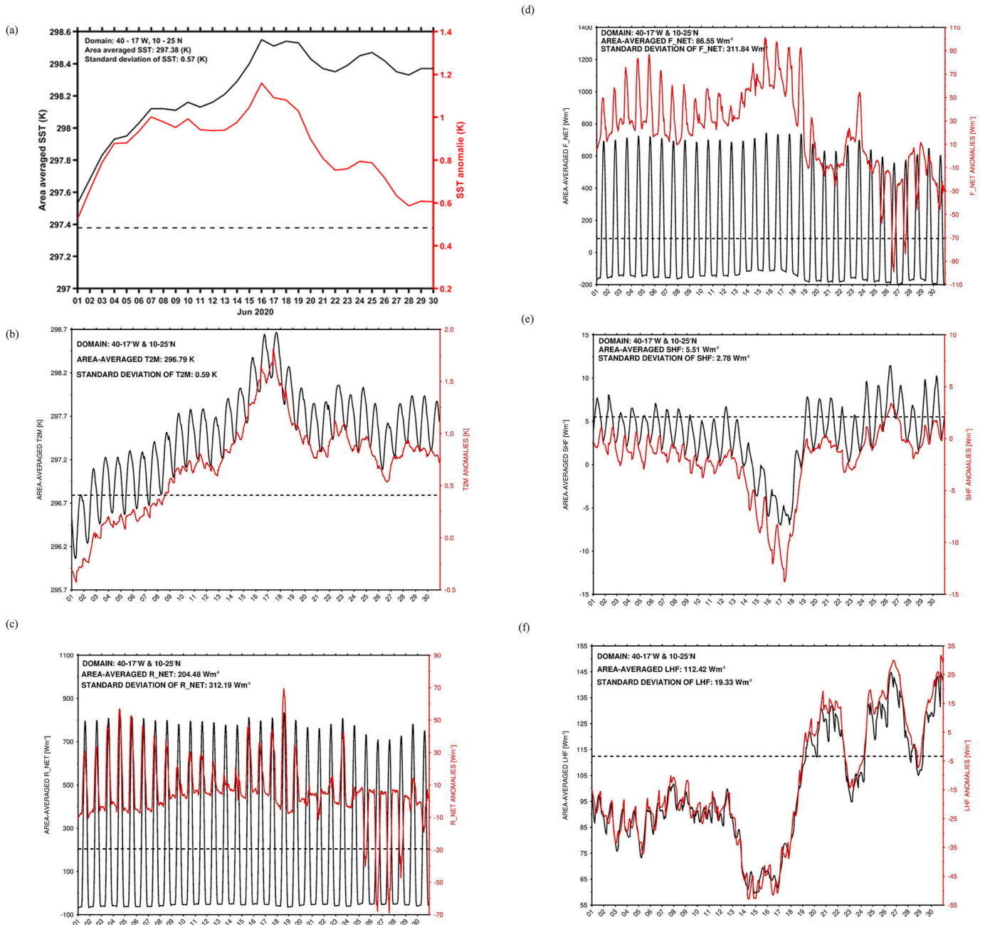
Fig. 6. Averaged over 40\text{--}17^\circ\text{W} & 10\text{--}25^\circ\text{N} (black rectangle in Fig. 1) for the June 2020 actual values and anomalies of (a) Daily SSTs (K) from GHRSSST, and ERA-5 (b) 2-m temperature (K), (c) total radiation flux ( R_{\text{net}} ), (d) total energy flux ( F_{\text{net}} ) at the surface in \text{W m}^{-2} (both positive if downward into the surface), (e) sensible heat flux (SHF) and (f) latent heat flux (LHF) in \text{W m}^{-2} (both positive if upwards into the atmosphere). The GHRSSST anomalies are computed with respect to the 2002–2019 climatology, while those of ERA-5 are with respect to the 2000–2019 climatology, as GHRSSST data is not available prior to 2002. In all panels, the climatological mean and standard deviation are given at the top left, with the former also plotted as a dashed line.
