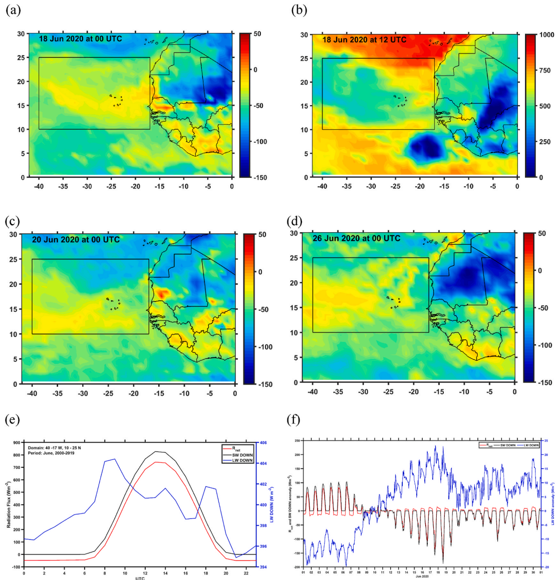
Fig. 4. CERES net radiation flux at the surface, R_{net} (W m -2 ), on 18 June 2020 at (a) 00 UTC and (b) 12 UTC; at 00 UTC on (c) 20 June 2020 and (d) 26 June 2020. (e) Climatological diurnal variation of area-averaged CERES downward short-wave and long-wave and R_{net} fluxes over the black rectangle in Fig. 1a. (f) is as (e) but showing the hourly anomalies for the month of June 2020.
