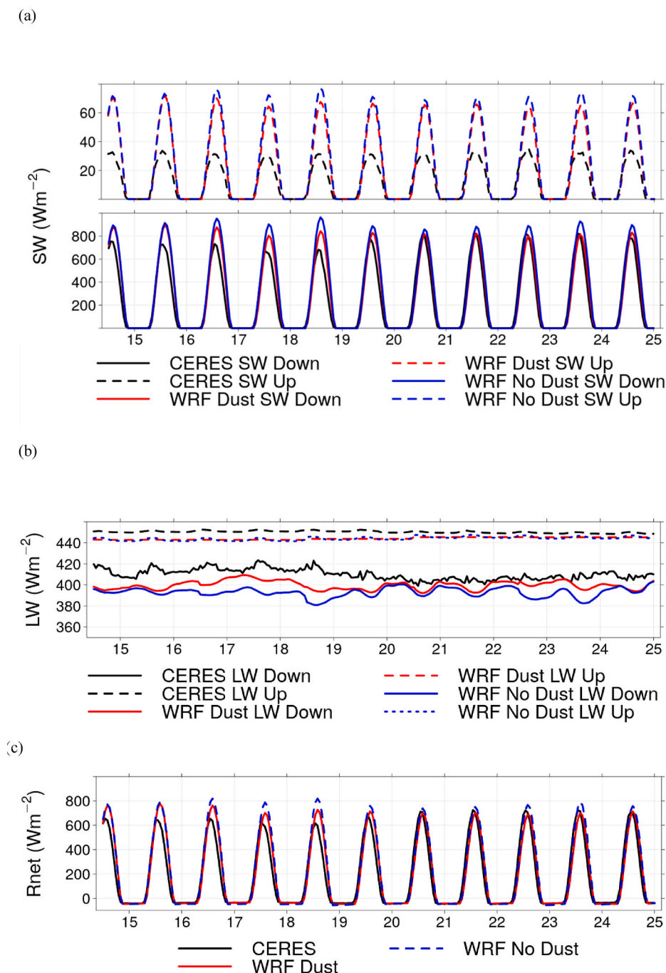
Fig. 5. Time series of the upward (dashed line) and downward (solid line) (a) shortwave and (b) longwave radiative fluxes, and (c) net radiative flux (R net ; W m -2 ) from WRF (red) and CERES (black) averaged over 38°W-17°W & 10°N-25°N and for the period 14-24 June 2020. The predictions of the WRF simulations in which the DRE is accounted for are given by red lines, and those of the run without DRE are plotted in blue lines. (For interpretation of the references to colour in this figure legend, the reader is referred to the Web version of this article.)
