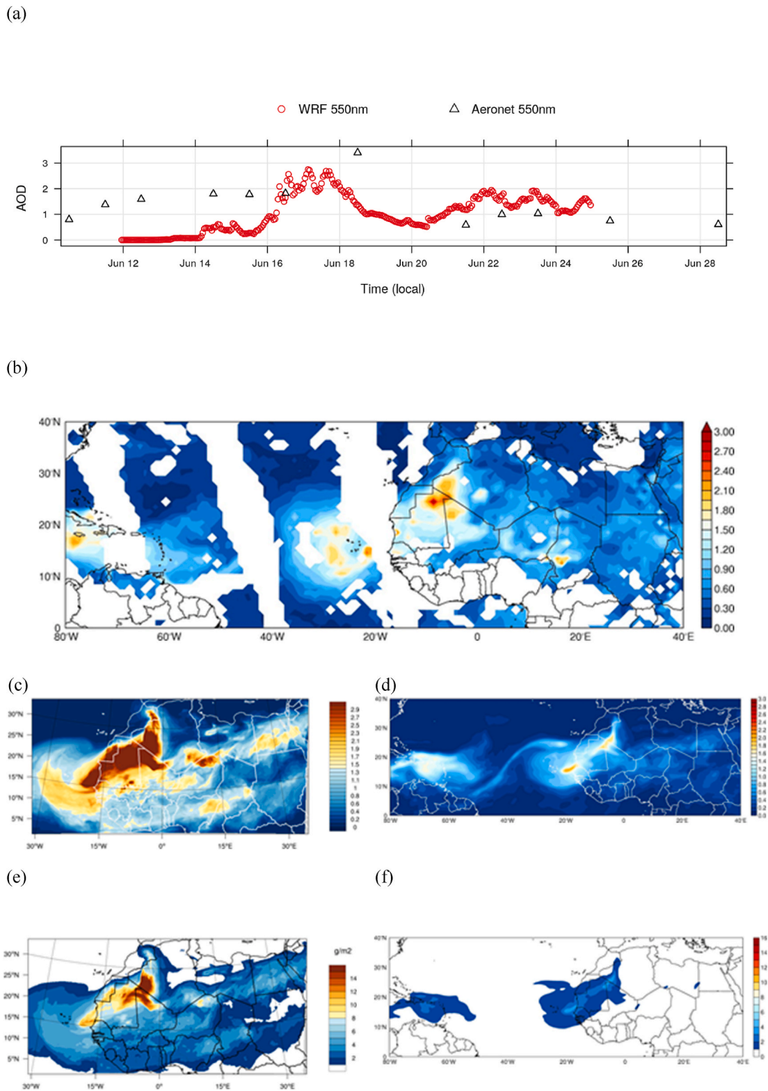
Fig. 3. As Fig. 2 but on 23 June 2020. In (a), the WRF and observed AOD at 550 nm from 10 to 29 June 2020 are plotted at the location of the AERONET station in Cape Verde ( 22.935^\circ\text{W} , 16.733^\circ\text{N} ). The western boundary in the VIIRS and MERRA-2 plots, panels (b), (d) and (f), is extended to 80^\circ\text{W} , to highlight the propagation of the dust plume into the Caribbean and North America.
