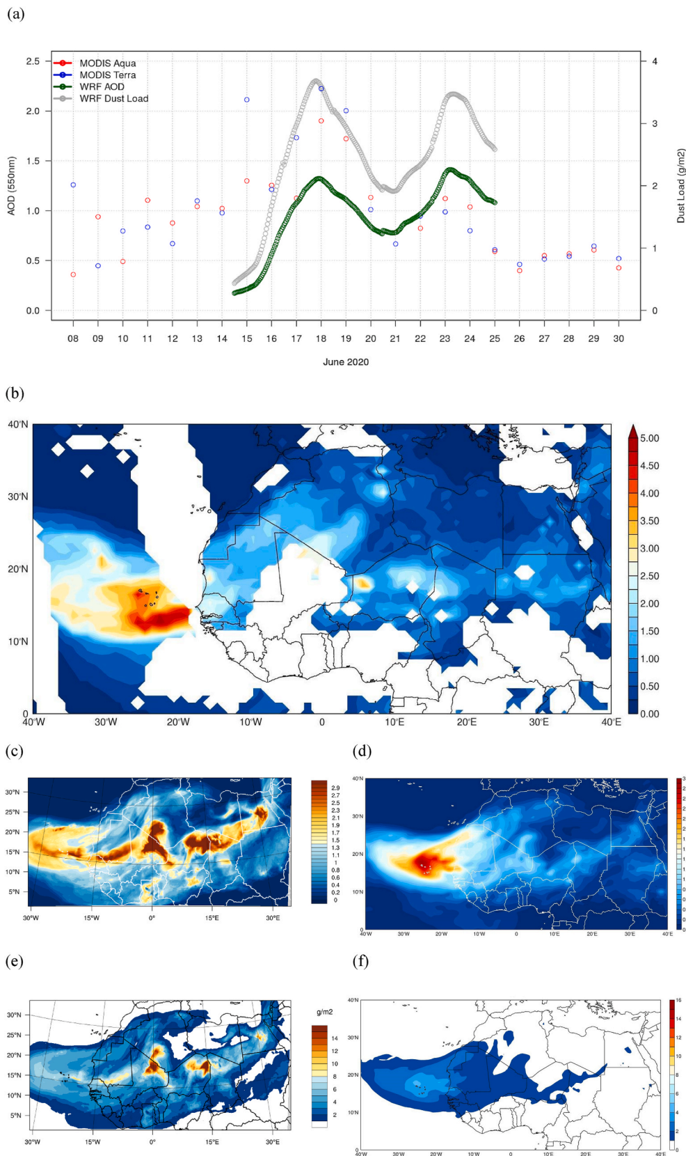
Fig. 2. (a) WRF AOD (green circles, left axis) and dust load (grey circles, right axis; \text{g m}^{-2} ) and MODIS AOD (blue and red circles; left axis), averaged over the eastern tropical Atlantic Ocean ( 38^{\circ}\text{W} - 17^{\circ}\text{W} & 10^{\circ}\text{N} - 25^{\circ}\text{N} ), from 08 to 30 June 2020. Spatial distribution of the AOD over the study region on 18 June 2020 from (b) VIIRS satellite (daily maximum; the white shading denotes gaps in the data coverage), (c) WRF and (d) MERRA-2 at 00 UTC. (e) and (f) are as (c) and (d) but for the total column dust mass ( \text{g m}^{-2} ). (For interpretation of the references to colour in this figure legend, the reader is referred to the Web version of this article.)
