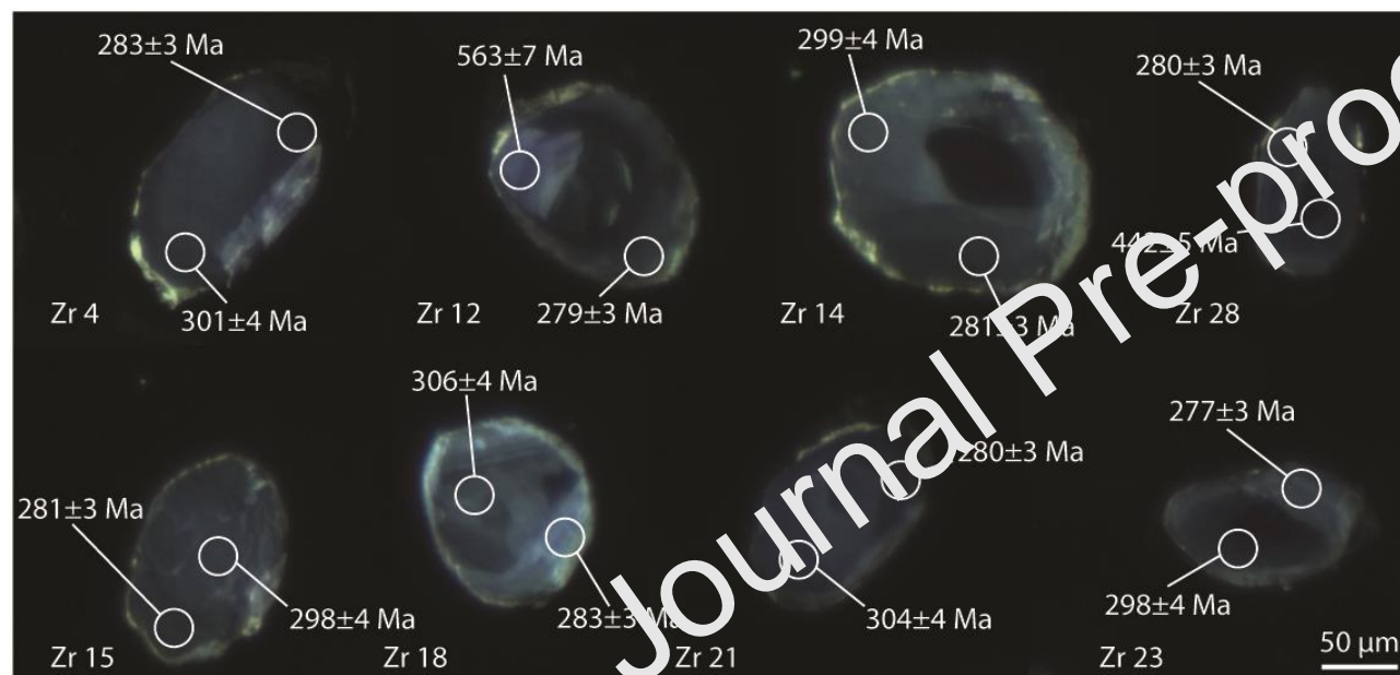
Fig. 12: Representative cathodoluminescence images of the dated zircon grains from the Saleix tonalite (Sample Sal-E). Morphology varies from euhedral to subhedral, with rare anhedral crystals. Zircon crystals dominantly show oscillatory cores with brighter overgrowths at the rims. White circles show the location of LA-ICP-MS spots with the relative ^{206}\text{Pb}/^{238}\text{U} ages and their 1\sigma error (see Table ST8 for details). Note that rim ages are always ~280 Ma.
