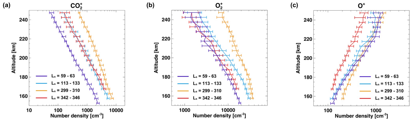
Figure 5. Median vertical profiles of ion species, as shown in Figure 4. (a) \text{CO}_2^+ , (b) \text{O}_2^+ , and (c) \text{O}^+ densities.
