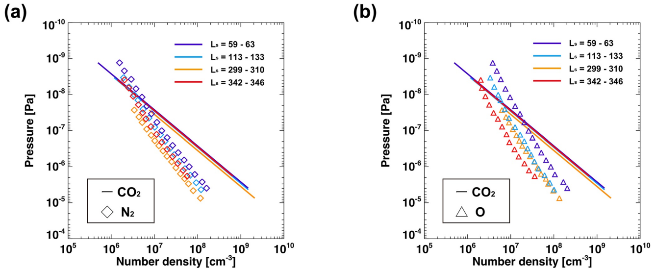
Figure 9. Vertical profiles of neutral species shown in Figure 4 are replaced with pressure coordinates. The pressure level is derived from the \text{CO}_2 density and its scale height. The lines are the median \text{CO}_2 densities. Diamonds in (a) are the median \text{N}_2 densities, and triangles in (b) are the median O densities. Each profile is distinguished by color as in Figure 4.
