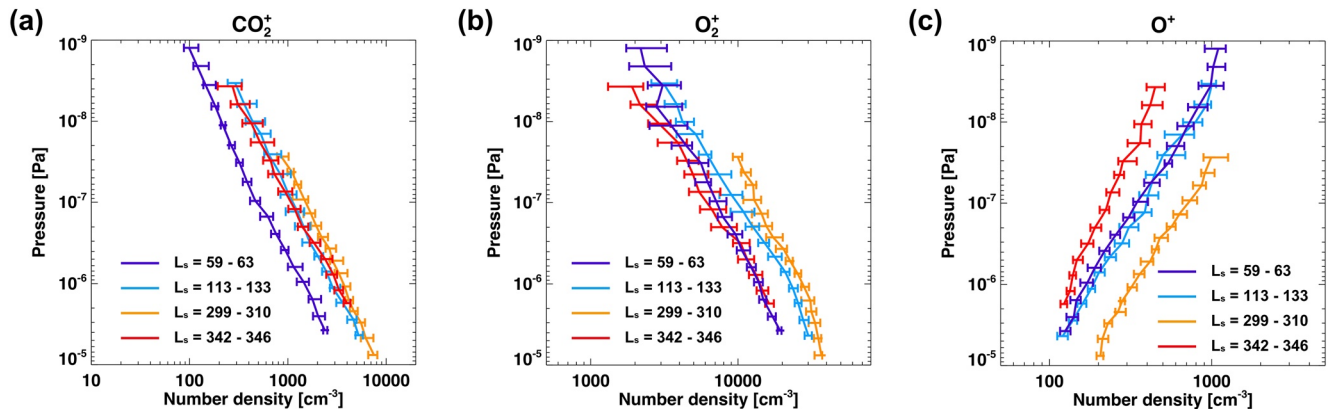
Figure 10. Vertical profiles of ion species shown in Figure 5 are replaced with neutral pressure coordinates.
