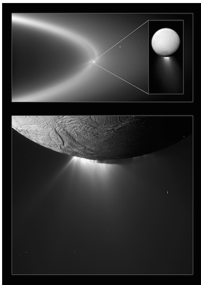
Figure 2.3.3: Cassini ISS images of Enceladus' eruption activity from different distances, illustrating that the ejected icy particles feed the E-Ring (top) Credits: NASA/JPL/SSI.
