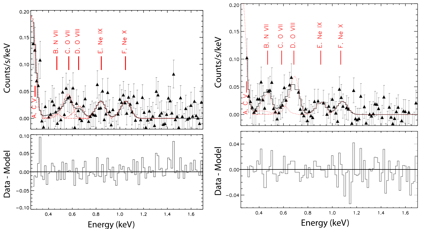
Figure 7. Chandra/ACIS-S3 spectra of comet 46P for epoch 1 (left panel) and epoch 2 (right panel). Each figure shows the background-subtracted spectrum overlaid with the best fitting emission line model with the residuals (model subtracted from the data) shown below. The model consists of six Gaussian components for both epochs 1 and 2. Individual Gaussian components are over-plotted in each panel as red dotted lines, and line IDs are indicated.
