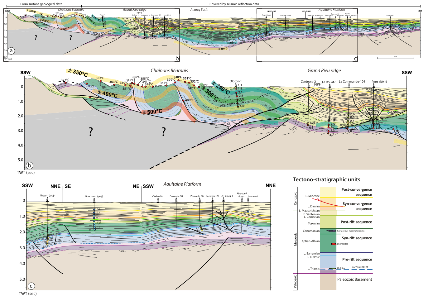
Fig. 9. N-S geological cross-section across the Western Pyrenées (see location on Fig. 1) associated with measured T_{\max} and Vitrinite Reflectance data. The southern part of the section drawn from surface geology is modified from Labaume and Teixell (2020). According to the seismic reflection data, the vertical scale of the whole section is in two-way traveltimes (second). To preserve coherency within the whole section, the southern part of the section constructed with surface geology was drawn in the prolongation of the seismic data based on TWT vertical-scale. (a) 100 km-long N-S stiking geological cross-section through the Chaînons Béarnais, Grand Rieu ridge, Arzacq Basin and the Aquitaine platform, built from a 2D reflection seismic composite line available in Figure S1. (b) close-up focused on the Chaînons Béarnais and the Grand Rieu ridge. (c) close-up focused on the Aquitaine platform.
