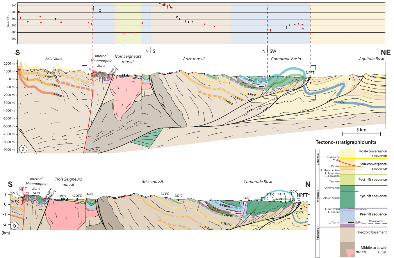
Fig. 10. N-S-striking geological cross-section (see location on Fig. 1) across the Central Pyrénées from the Axial Zone to the south to the Aquitaine Foreland Basin to the north. (a) Geologic cross-section associated with the distribution of the HT/LP metamorphism and relevant graph ( T_{max} versus distance). The isograds were plotted with a margin of error. (b) Close-up on the Mesozoic basins.
