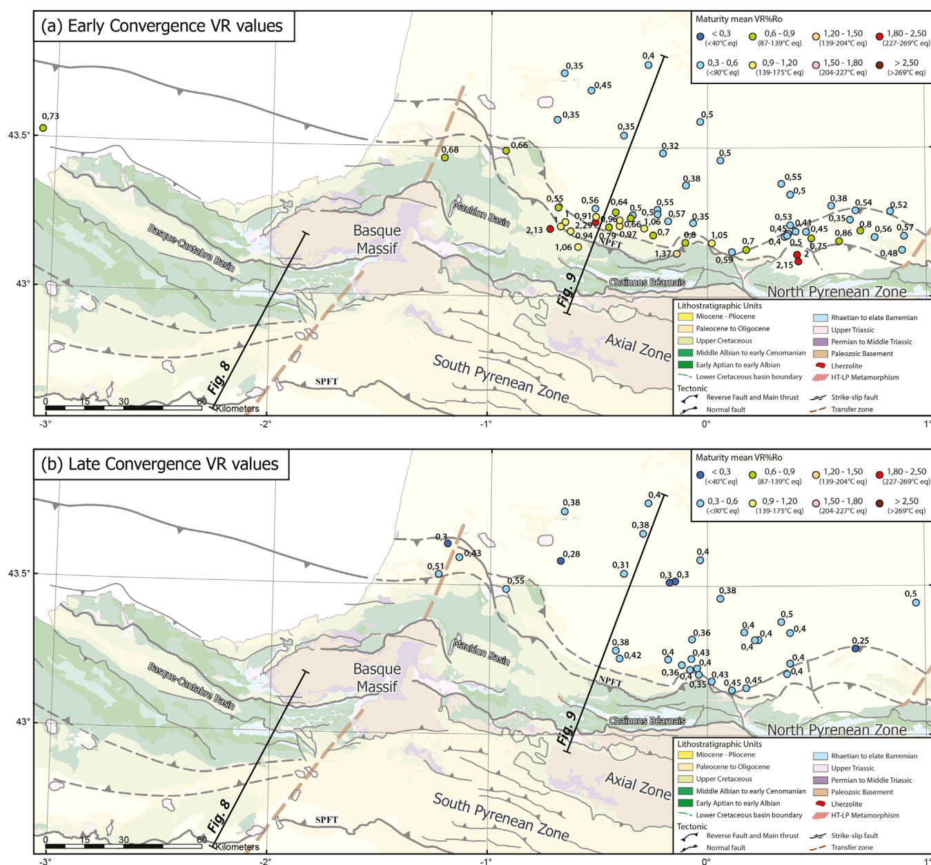
Fig. 4. Maps displaying the spatial distribution of R_0 data for each convergence-related tectono-stratigraphic unit. (a) average R_0 values measured in early-convergence sediments (Santonian to Maastrichtian). (b) average R_0 values measured in later-convergence sediments (Danian to Chattian).
