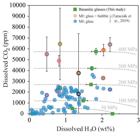
Figure 12. Comparison between H 2 O–CO 2 contents from olivine- and clinopyroxene-hosted basanite melt inclusions from El Hierro, Canary Islands [Taracsák et al. , 2019] and the H 2 O–CO 2 solubility curves ( dashed lines ) determined for our basanitic melt ( green squares ) at pressures from 50 MPa to 400 MPa. Light blue circles represent MI glass phases and orange circles correspond to reconstructed melt inclusions (bubble + glass). Coloured borders indicate pairs of unreconstructed and reconstructed MI. Most melt inclusions (glass phases) are located between the 100–200 MPa isobars (equivalent to 3–6 km), whereas the restored MI gives higher pressures (280–440 MPa).
