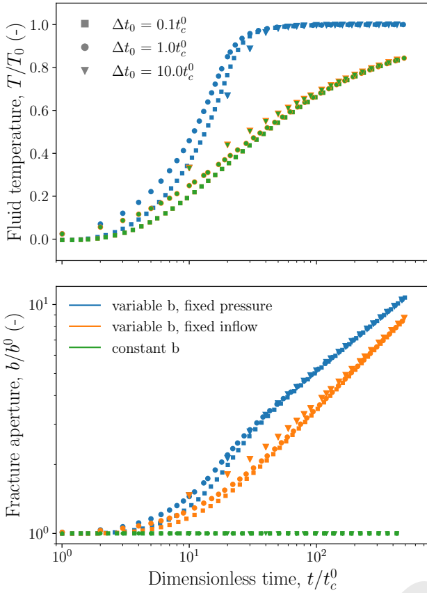
Figure 5: Temporal evolution of fluid temperature (top) and semi-aperture (bottom) for a fracture subject to cold fluid injection. Results correspond to a control plane placed at 3.5 m from the injection section at x = 0 . The case with constant fracture aperture and velocity (green) is compared with the case of temperature dependent fracture aperture and velocity, under the inlet BC of constant pressure (blue) or constant inflow (orange). The different markers correspond to different values of the time interval, from 0.1 to 10 times the initial characteristic time t_c^0 , as defined in the text. Fluid temperature is normalized with respect to the temperature injected at the inlet, semi-aperture is normalized with respect to its initial value, while time is normalized with respect to t_c^0 . Marker plot-frequency is adjusted to improve visualization.
