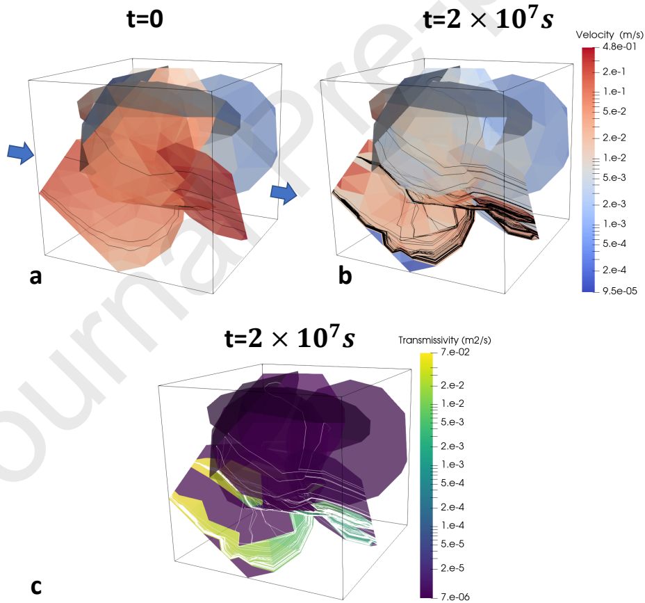
Figure 11: Velocity field at the initial time (a), velocity (b) and transmissivity (c) fields at time equal to 2 \times 10^7 s in the example DFN with temperature-dependent fracture aperture under the continuous injection of 4 particles in the system. Black and white lines represent the trajectories of the particles injected until the represented time, where the color is solely chosen for visualization purposes. The arrows in (a) indicate the fluid inlet and outlet sections.
