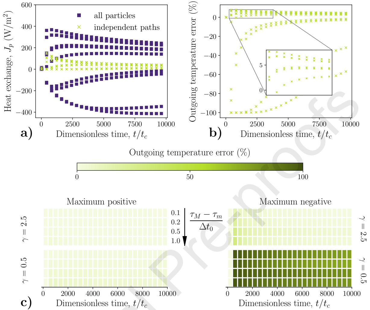
Figure 9: a) Diffusive fluid/rock heat flux, J_p , undergone by each particle at different times, evaluated considering the contribution of all particles taken individually (eqs. (28) and (29), blue squares), and the contribution of the single particle under the assumption of independent flow paths (eq. (38), green crosses). Each marker corresponds to one particle. The same set of 10 particles arrive at the control location at each t_0 with stationary passage times \tau following a power law pdf distribution and temperatures proportional to \text{erfc}(\tau/\sqrt{t}) . b) Relative error in the estimation of the particle temperature after having exchanged J_p with the rock for a \Delta\tau=1 s when the assumption of independent flow paths is considered. c) Maximum values (averaged over 100 realizations) of positive and negative relative errors in the outgoing temperature when the assumption of independent flow paths is considered. Columns represent different observation times, rows represent different scenarios of values for the exponent of the passage time power law pdf distribution, \gamma , and for the time interval \Delta t_0 . The results shown in the top panels correspond to one of the realizations of the case with \gamma=0.5 and \Delta t_0 = \tau_M - \tau_m , represented in the last row of the colorplots. Time is normalized with respect to the characteristic time for the unitary \Delta\tau . For all plots, the writing frequency has been adjusted in order to show results at the same time for all cases. More details in Section 6.
