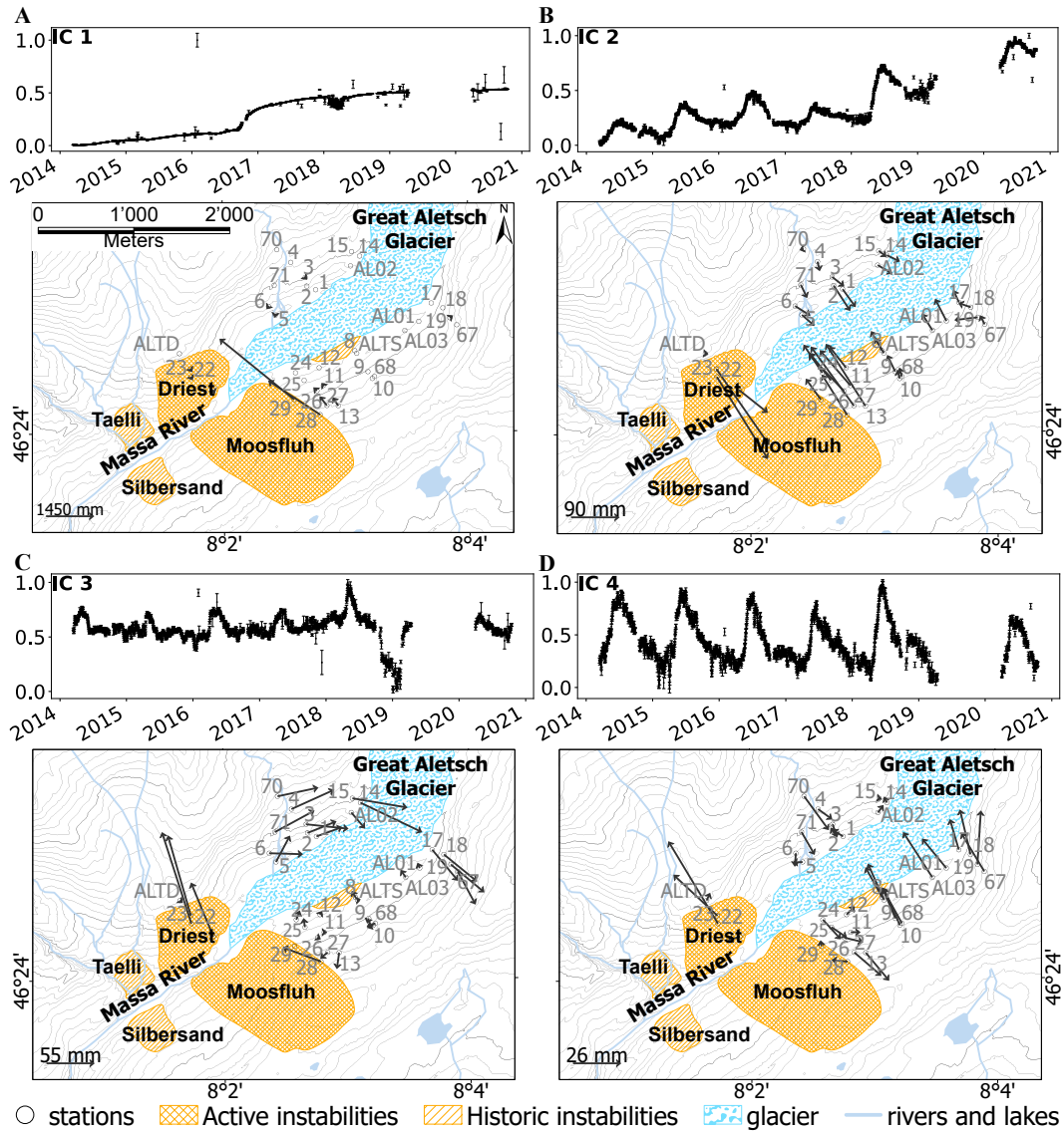
Figure 5. Results of the vbICA analysis with four independent components (A: IC1, B: IC2, C: IC3 and D: IC4). The temporal function of each component is shown above its respective spatial distribution at points included in the analysis (grey labels).
