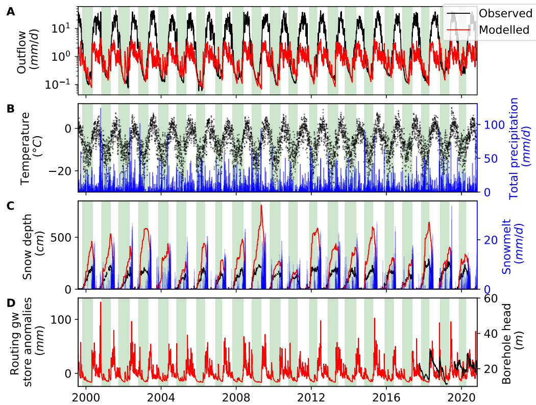
Figure 4. Results of the GR5J model for groundwater storage estimation at catchment scale. A: flow in the Massa river, normalized by the size of the catchment, with observations (black) and model (red). Calibration periods are shown in green. B: temperature at the Jungfrauoch station (black) and precipitation at the Fiesch station (blue). C: snow depth at the Eggishorn station (black), modeled from GR5J for the entire catchment (red) and modeled snowmelt (blue). D: anomalies to the mean of the groundwater storage modeled (red) and observed head in the borehole B4 (black).
