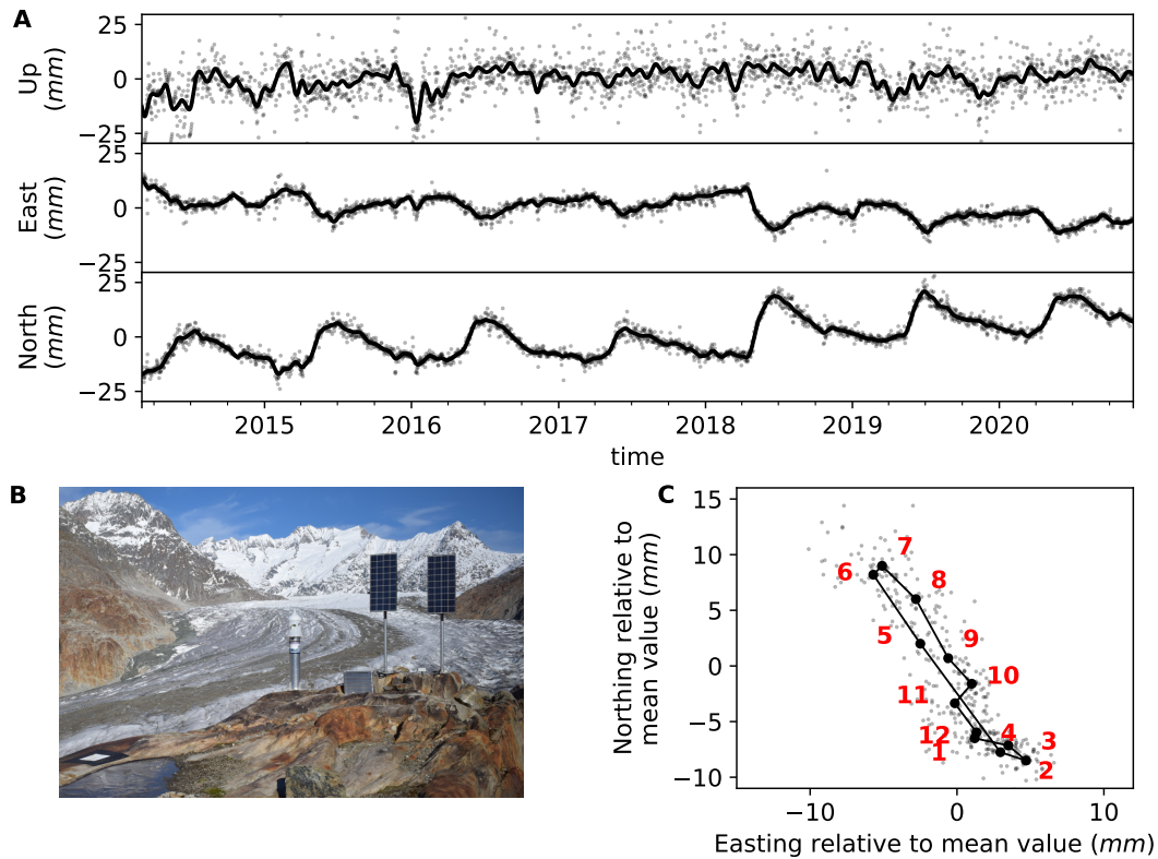
Figure 3. Example of time series for a cGPS situated at the Chazulecher station (ALTS). A: three spatial components of displacement relative to HOHT (grey dots) with filtered data (black line). B: picture of the station and its surroundings, view to NE. The GPS is on top of the total station (left mast). C: horizontal displacement seen from top. Grey points are average values from ordinal days after linear detrending of the time series. Black points are average monthly values, labeled in red. The quicker deformation in spring to early summer to the NNW is followed by a slower, more gradual deformation in the opposite direction during the rest of the year. The cyclic deformation is mainly in the horizontal direction, although the higher noise in the vertical component might prevent the detection of annual cyclicity.
