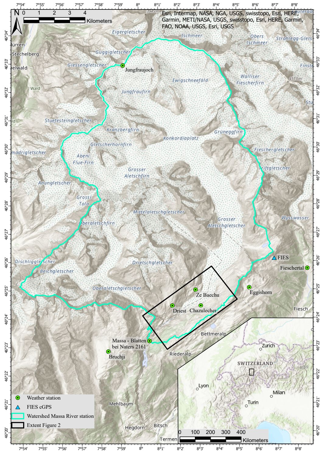
Figure 1. Topographic map of the central European Alps. The weather stations used (green points) and the cGPS station FIES (blue triangle) are shown. The black rectangle is the extent of Figure 2 and the inset shows the location of this map in the European Alps.
