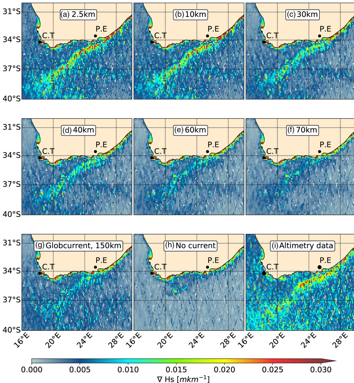
Figure 4. Significant wave height gradient ( \nabla H_s ) averaged over the years 2014–2016, from (a–h) model simulations and (i) altimeters data. \nabla H_s estimated along satellite tracks are gridded on a regular 1/8^\circ \times 1/8^\circ grid. Simulation with the original CROCO surface currents is represented in (a). Simulations forced with filtered surface currents at effective resolutions of 10, 30, 40, 60, and 70 km are displayed in panels (b), (c), (d), (e), and (f), respectively. The simulation with Globcurrent data is shown in (g) and the model result without any surface current forcing is shown in (h). CROCO, Coastal and Regional Ocean Community.
