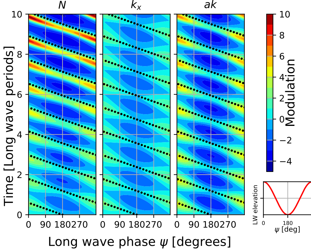
Figure 1. Evolution of short wave properties, action N , wavenumber k and slope ak , in the frame of reference moving with the long wave phase \psi , with \psi = 0 corresponding to the long wave crest. The short wave quantities are normalized by the long wave slope \varepsilon_L , following the definition of the modulation in eq. (12). The case shown here is for k_i/k_L = 10 , \varepsilon_L = 0.1 , \gamma_i = 1 and a Courant number Co=0.1 . starting with a uniform distribution of N and k at t = 0 . The black dots correspond to successive positions of a linear wave group starting from the trough of the long wave profile and propagating at apparent speed of the short wave groups 0.5C_i (see Appendix C).
