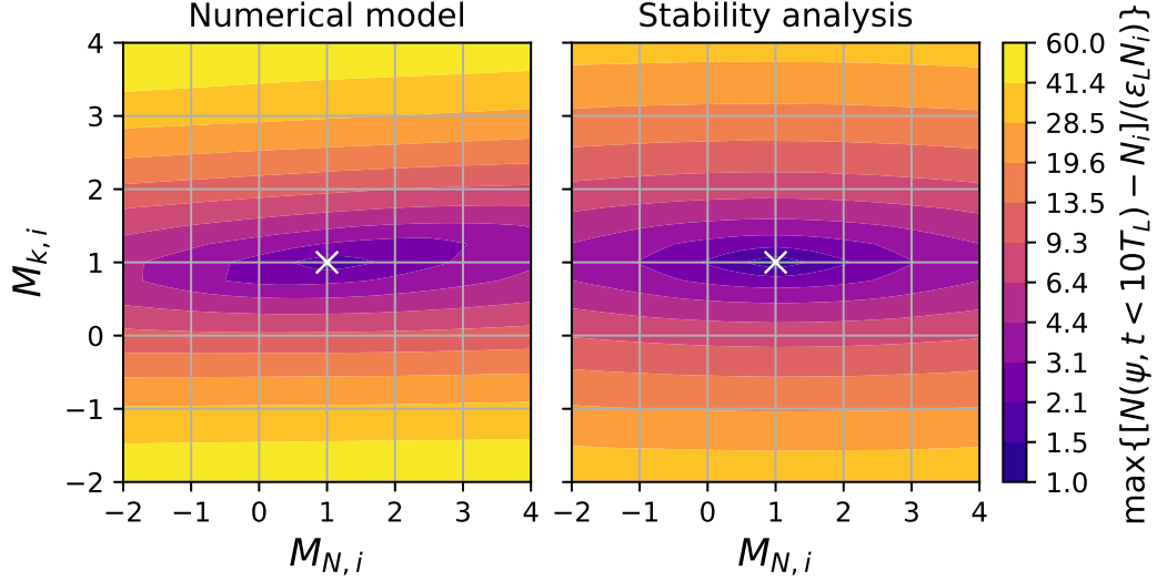
Figure 4. Maximum action modulation after 10 long wave periods from initiation as a function of various initial modulations. The runs are performed with k_i/k_L = 10 , \varepsilon_L = 0.1 , \gamma_i = 1 and \text{Co} = 1 . The white crosses stand for LH&S initial conditions M_{N,i} = M_{k,i} = 1 .
