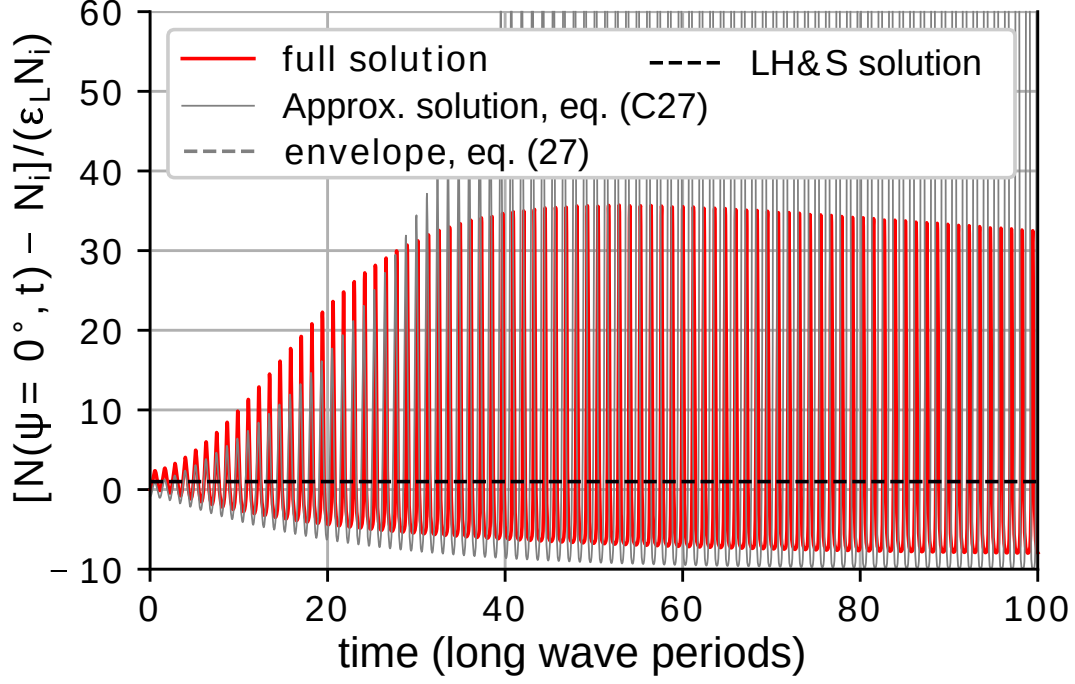
Figure 3. Wave action modulation on wave crests (same case as figure 2b for a longer time range).
