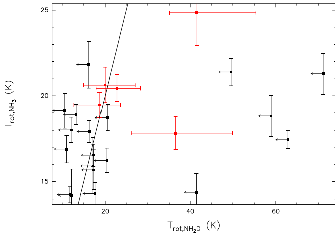
Fig. 5. Observed NH 3 rotational temperature between the (1,1) and (2,2) inversion transition is shown against modelled NH 2 D rotational temperature between the 1 11 –1 01 line at 110 GHz and the 2 12 –2 02 transition at 74 GHz. Sources with a detected 74 GHz line are marked in red, and non-detections with an upper limit of the NH 2 D temperature are labelled as black arrows. The straight line corresponds to equal temperatures.
