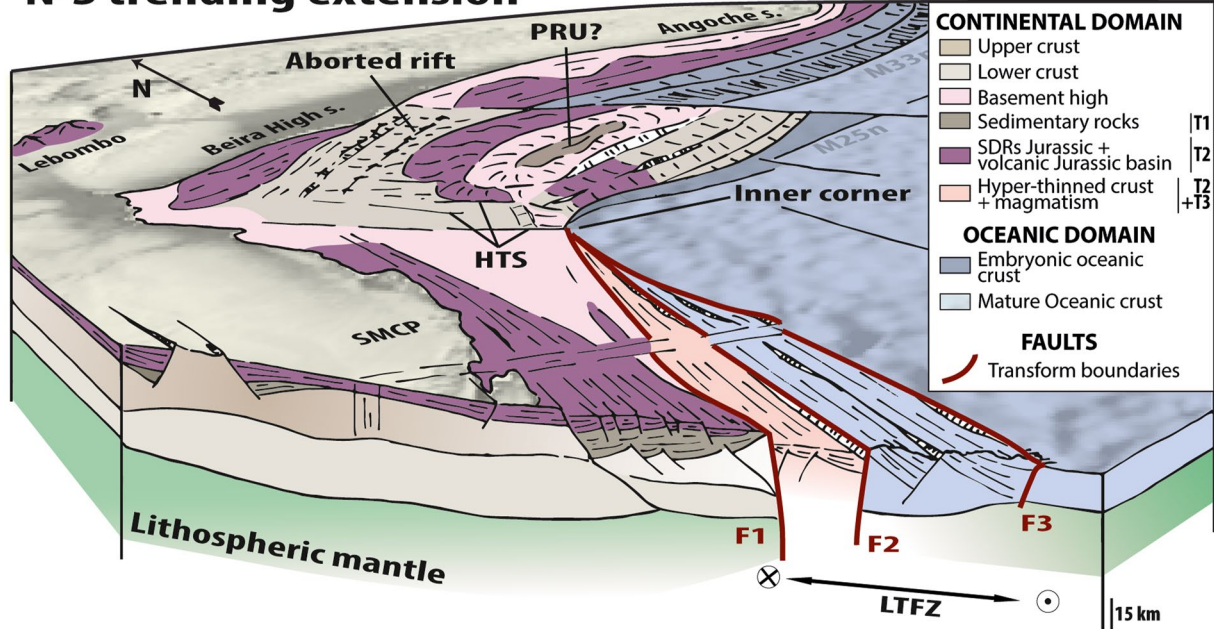
Figure 10. Synthetic 3D bloc diagram showing the basement structures, syn-rift deposits and magmatism during the transform stage that corresponds to the Limpopo transform margin activity. This sketch is consistent with our structural map in Figure 2 showing the segmentation of the Mozambique margins with, from west to east the Limpopo, the Beira High and Angoche margin segments. Horsetail Transfer Structures (HTS), Limpopo East (LE), Limpopo Main (LM), Limpopo Transform Fault Zone (LTFZ), Limpopo West (LW), Pre-Rift Unit (PRU), South Mozambique Coastal Plain (SMCP), Segment (s).
