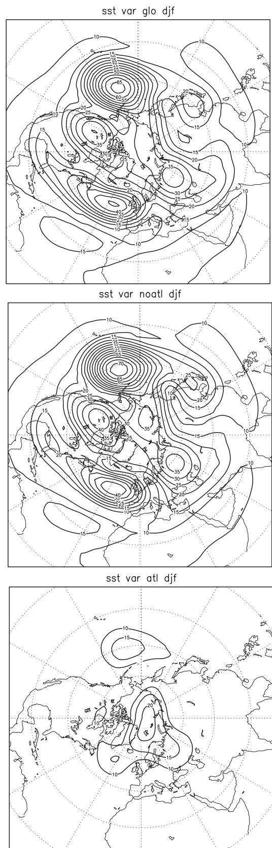
Fig. 3. Same as in fig. 1, but for the external forced variability.
