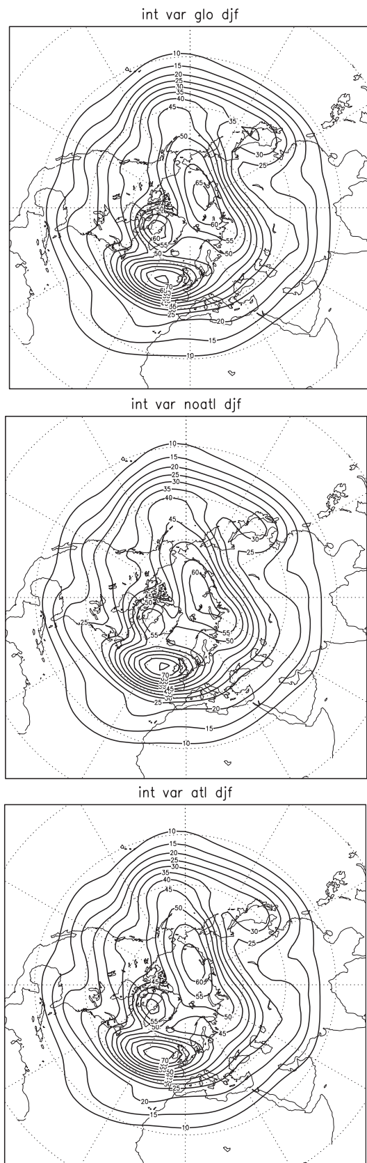
Fig. 2. Same as in fig. 1, but for the internal variability.
