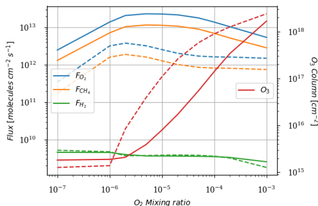
Figure 8. Surface oxygen ( F_{O_2} ) and methane ( F_{CH_4} ) fluxes, hydrogen escape ( F_{H_2} ) and O_3 column density as a function of surface O_2 for a surface CH_4 set up at 10^{-4} . Results for 1D model surface temperature 280K (solid) and 220K (dashed).
