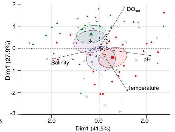
FIGURE 3 Principal component analysis of the monthly average conditions in bottom seawater at Sechura and Paracas. Biplots represent the two first principal components with 60.39 and 69.38% of the total variability explained in Sechura and Paracas, respectively. DO_{sat} : dissolved oxygen saturation; Sal: salinity; Temp: temperature. There were significant differences ( p < .0001 ) between the ENSO phases and seasons at both sites. Ellipses indicate 95% confidence limits of the seasonal average bottom-water-condition groupings
