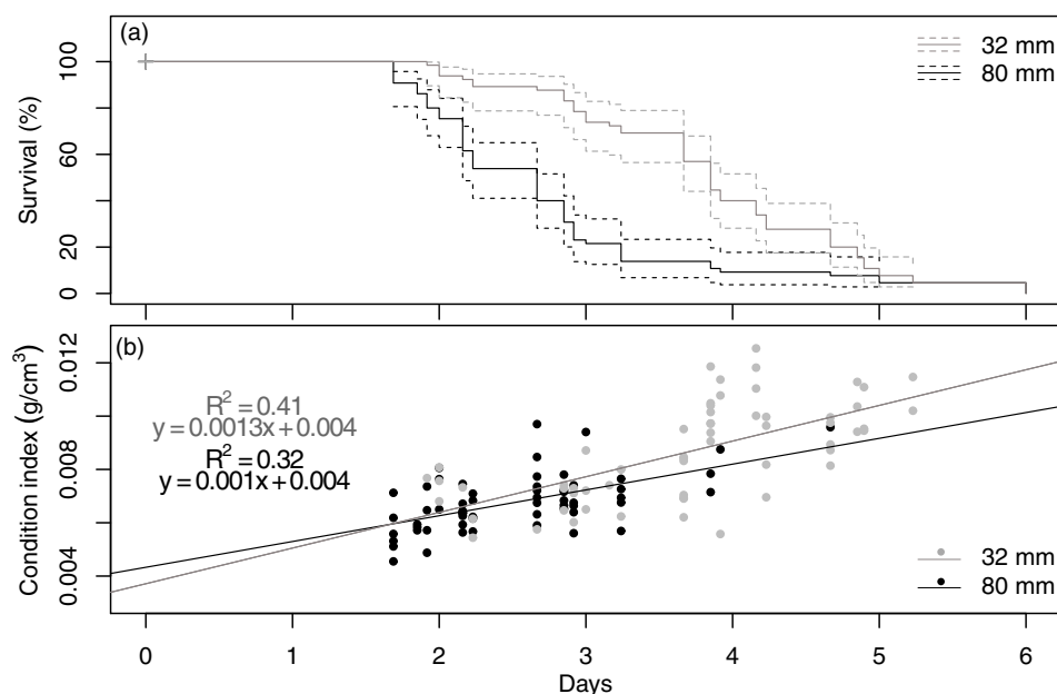
FIGURE 6 Survival of small- and large-sized groups of Argopecten purpuratus at 1% DO sat : (a) survival curves and (b) the relationship between individual survival time and condition index. Dashed and dotted lines represent 95% confidence intervals and the median lethal time, respectively. Linear regression models represent the significant positive relationships ( p < .0001 ) between the survival time and condition index in both size groups
