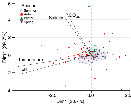
FIGURE 3 Principal component analysis of the monthly average conditions in bottom seawater at Sechura and Paracas. Biplots represent the two first principal components with 60.39 and 69.38% of the total variability explained in Sechura and Paracas, respectively. DO_{sat} : dissolved oxygen saturation; Sal: salinity; Temp: temperature. There were significant differences ( p < .0001 ) between the ENSO phases and seasons at both sites. Ellipses indicate 95% confidence limits of the seasonal average bottom-water-condition groupings
