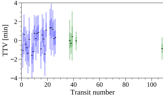
Fig. 7. TOI-674b transit-timing variations from TESS data (blue) and follow-up observations (green). The different shades of color of the error bars represent the 1\sigma (dark) and 3\sigma (light) levels of uncertainty of the measurements. No significant TTVs are detected in the \sim 200 days of baseline covered by the observations.
