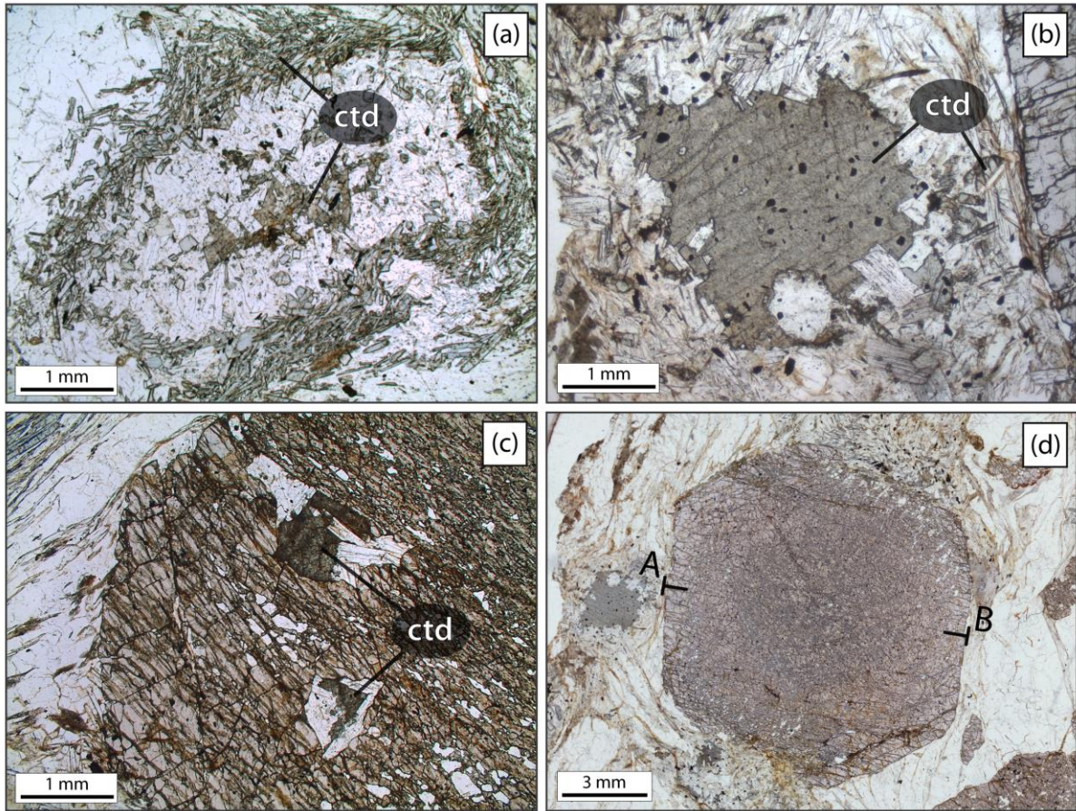
Figure 6. Thin section photomicrographs for sample GM1 (PPL). (a, b) Pseudomorphs after staurolite, consisting of a fine-grained chloritoid aggregate surrounded by white mica + chloritoid and a cluster of chloritoid. (c) Pseudomorph after staurolite included in garnet rim. Garnet rim preserves an internal foliation mainly defined by elongate quartz inclusions and oriented at high angle with respect to the matrix foliation. (d) Centimetre-sized pre-Alpine garnet porphyroblast. The A-B markers indicate the position of the compositional profile in Figure 7a.
