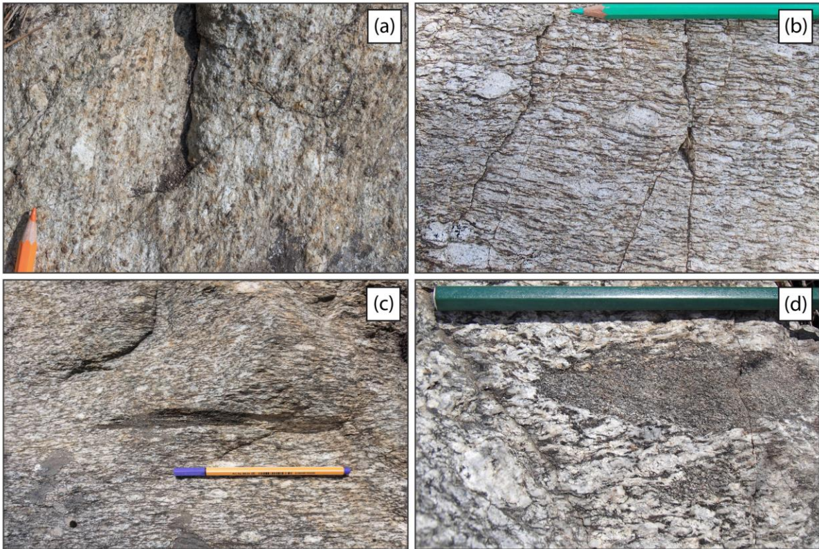
Figure 3. Field photographs of the Muret orthogneiss. (a) Garnet, up to 5 mm in size, dispersed in the Muret orthogneiss. (b) Orthogneiss with a pre-Alpine metamorphic foliation defined by the preferred orientation of biotite and white mica. Alkali feldspar porphyroclasts are elongated parallel to the pre-Alpine metamorphic foliation. (c) Highly stretched mafic enclave oriented parallel to the pre-Alpine metamorphic foliation. (d) Lenticular-shaped mafic enclave consisting of fine-grained biotite and minor feldspars.
