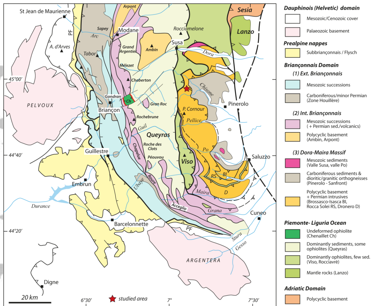
Figure 2. Simplified geological map of the SW Alps, showing the location of the studied area in the Dora-Maira Massif (modified after Ballèvre et al., 2020).
