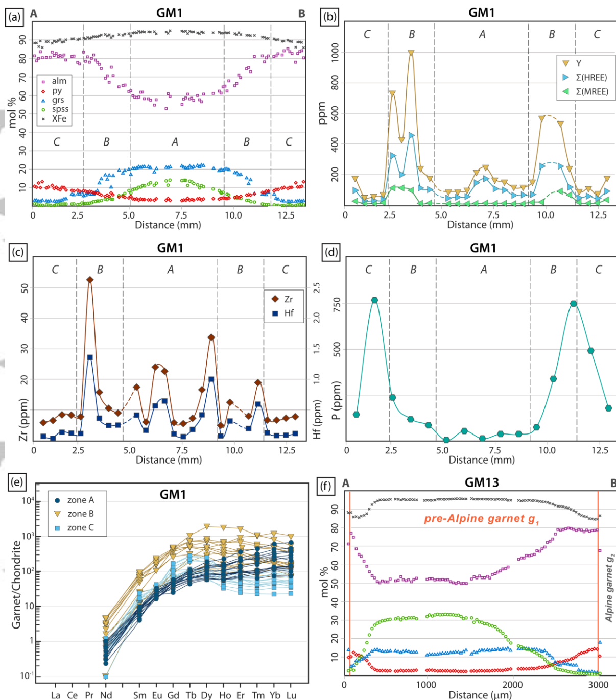
Figure 7. Compositional profile of pre-Alpine garnet from garnet-staurolite micaschist (GM1) for major (a) and trace elements (b, c, d). (b) Compositional profile of Y and sum of HREE and MREE. (c) Compositional profile of Zr and Hf. (d) Compositional profile of P. (e) Chondrite-normalized REE pattern (McDonough & Sun, 1995) for pre-Alpine garnet in sample GM1. (f) Compositional profile of polycyclic garnet from garnet micaschist (GM13) (color coding as in (a)). Vertical orange lines mark the boundaries between the first and second garnet generations. The position of the profiles (a) and (f) is indicated in Figure 6d and Figure 8e, respectively (lines A-B).
