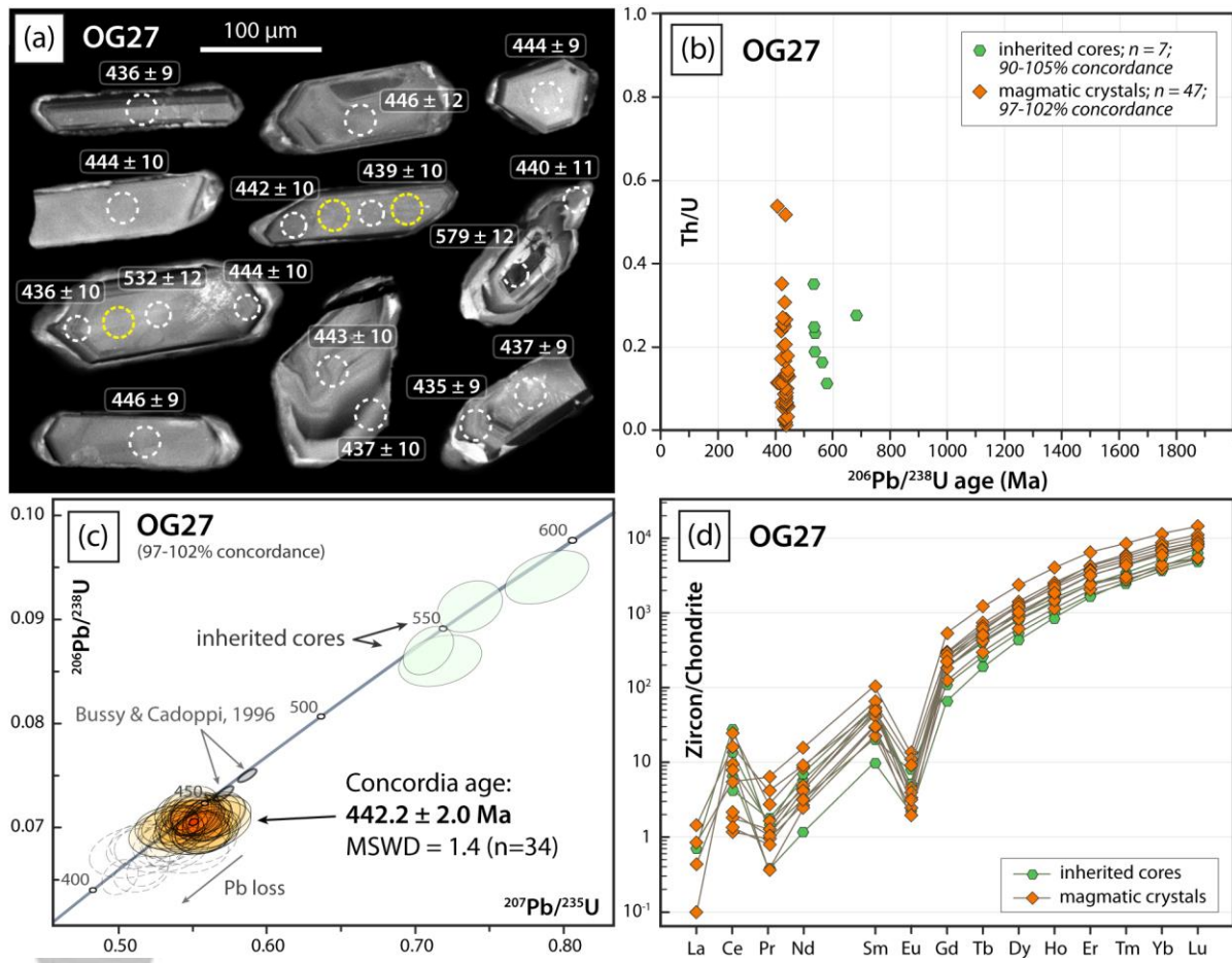
Figure 11. (a) Cathodoluminescence images of zircon from orthogneiss sample OG27. Dashed white and yellow circles represent the location of the LA-ICP-MS U-Pb (given as ^{206}\text{Pb}/^{238}\text{U} ages) and trace elements analyses, respectively. (b) Th/U ratio versus age plot for sample OG27. (c) Concordia diagram for zircon from sample OG27. Green ellipses indicate dates from inherited cores, whereas yellow ellipses indicate dates from magmatic crystals. Empty dashed ellipses represent dates excluded from magmatic Concordia age calculation. (d) Zircon trace element composition for sample OG27. REE patterns are normalized to chondrite values (McDonough and Sun, 1995).
