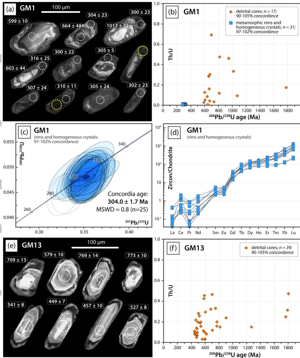
Figure 12. (a) Cathodoluminescence images of zircon from garnet-staurolite sample GM1. Dashed white and yellow circles represent the location of the LA-ICP-MS U-Pb (given as ^{206}\text{Pb}/^{238}\text{U} ages) and trace elements analyses respectively. Zircons in the first and second row display core and rim domains whereas zircons in the bottom row are internally homogeneous. (b) Th/U ratio versus age plot for sample GM1. (c) Concordia diagram for zircon dates (metamorphic rims and crystals) for sample GM1. Empty dashed ellipses represent data excluded from Concordia age calculation. (d) Trace element compositions of metamorphic zircon rims and homogeneous crystals for garnet-staurolite sample GM1. REE patterns are normalized to chondrite values (McDonough and Sun, 1995). (e) Cathodoluminescence images of zircon from garnet micaschist sample GM13. Dashed white circles represent the location of the LA-ICP-MS U-Pb analyses (given as ^{206}\text{Pb}/^{238}\text{U} ages). (f) Th/U ratio versus age plot for zircon from garnet micaschist sample GM13.
