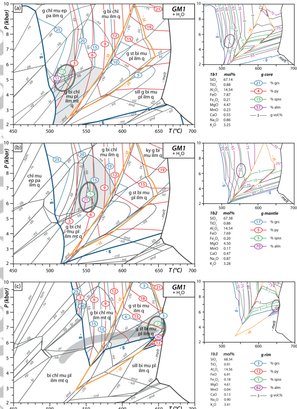
Figure 9. P – T pseudosections calculated for the garnet-staurolite micaschist GM1, considering progressive garnet fractionation. Some fields are not labelled for the sake of clarity; their assemblages can be deduced from assemblages in adjacent fields. The garnet-in, staurolite-in and melt-in lines (wet solidus) are highlighted with thick blue, orange and black lines, respectively. Grey circles indicate the P – T conditions at the three stages of garnet growth. (a) Pseudosection calculated for the bulk composition 1b1 (obtained by XRF) and used for constraining the P – T conditions of equilibration of garnet core. Garnet isomodes are shown in the small plot on the right-hand side. (b) Pseudosection calculated for the bulk composition 1b2 (after garnet core fractionation) and used for constraining the P – T conditions of equilibration of garnet mantle. (c) Pseudosection calculated for the bulk composition 1b3 (after garnet core and mantle fractionation) and used for constraining the P – T conditions of equilibration of garnet rim. The grey arrow indicates the P – T evolution as inferred from the three pseudosections.
