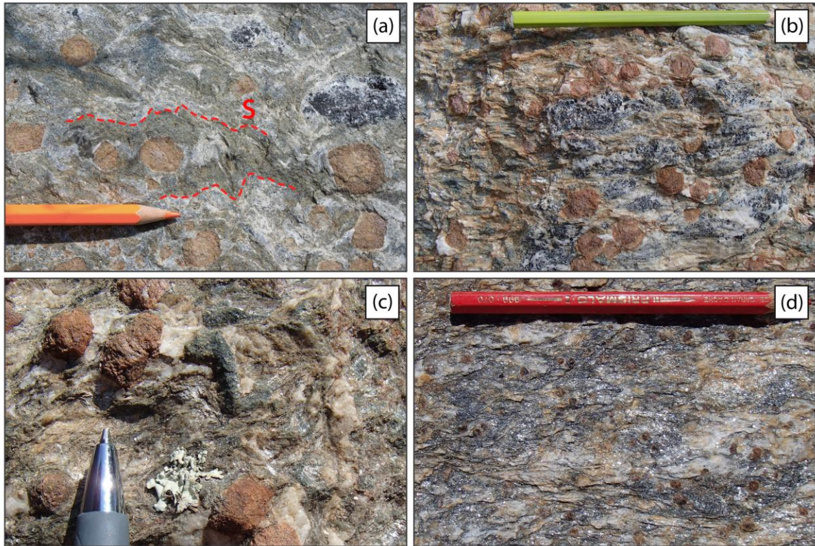
Figure 4. Field photographs of garnet-staurolite micaschist (a, b, c) and garnet micaschist (d) of the Punta Muret Unit. (a) Micaschist displays pre-Alpine garnet porphyroblasts and a pre-Alpine foliation defined by the alternation of quartz- and mica-rich layers (marked by red dashed lines). This structure is crenulated during the Alpine evolution. At the top right corner of the photograph are cm-sized veins and nodules of tourmaline and quartz. (b) Tourmaline-quartz veins oriented parallel to the pre-Alpine foliation. (c) Pseudomorph after staurolite with preserved prismatic crystallographic faces. (d) Grey-coloured garnet micaschist cropping out outside the low-strain domain.
