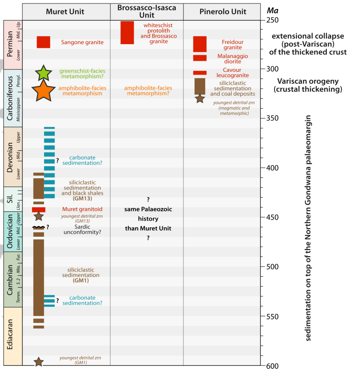
Figure 15. A summary of the pre-Alpine evolution of the Dora-Maira Massif. See text for further explanation.
