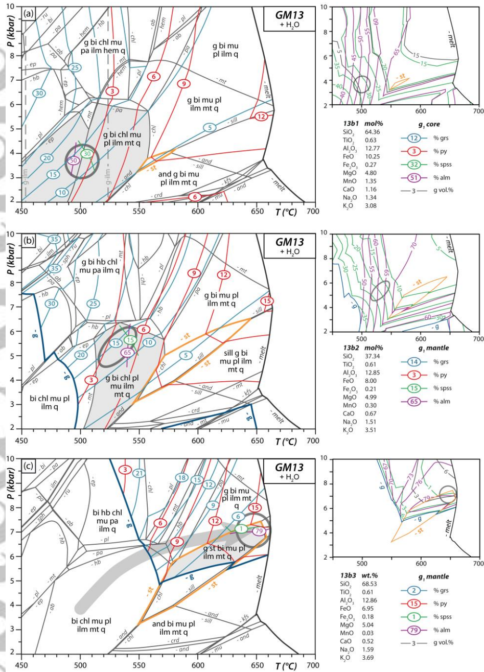
Figure 10. P – T pseudosections calculated for the garnet micaschist GM13, considering progressive garnet fractionation. Some fields are labelled for the sake of clarity; their assemblages can be deduced from assemblages in adjacent fields. The garnet-in, staurolite-in and melt-in lines (wet solidus) are highlighted with thick blue, orange and black lines, respectively. Garnet composition is used to constrain the P – T conditions (indicated by a grey circle) at the three stages of garnet growth. (a) Pseudosection calculated for the local bulk composition 13b1 (obtained by area scan method) and used for constraining the P – T conditions of equilibration of garnet 1 core. Garnet isomodes are shown in the small plot on the right-hand side. (b) Pseudosection calculated for the bulk composition 13b2 (after garnet 1 core fractionation) and used for constraining the P – T conditions of equilibration of garnet 1 mantle. (c) Pseudosection calculated for the bulk composition 13b3 (after garnet 1 core and mantle fractionation) and used for constraining the P – T conditions of equilibration of garnet 1 rim. The grey arrow indicates the P – T evolution as inferred from the three pseudosections.
