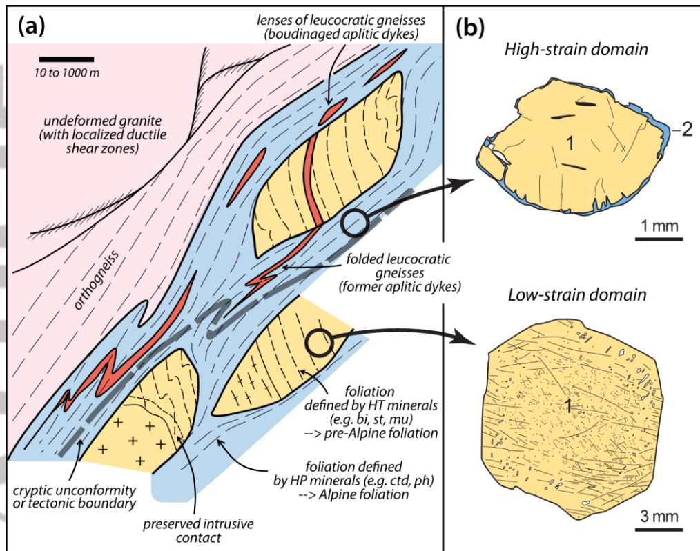
Figure 1. (a) Schematic representation of the strain patterns in a polycyclic basement. Low-strain volumes preserving structures and minerals from a first orogenic cycle (yellow) are bounded by rocks fully reworked during a second orogenic cycle (pale blue). (b) Garnet in low-strain domains may preserve their shape, inclusions, and chemical zoning while garnet in the high-strain domains may display overgrowths related to the second orogenic cycle.
