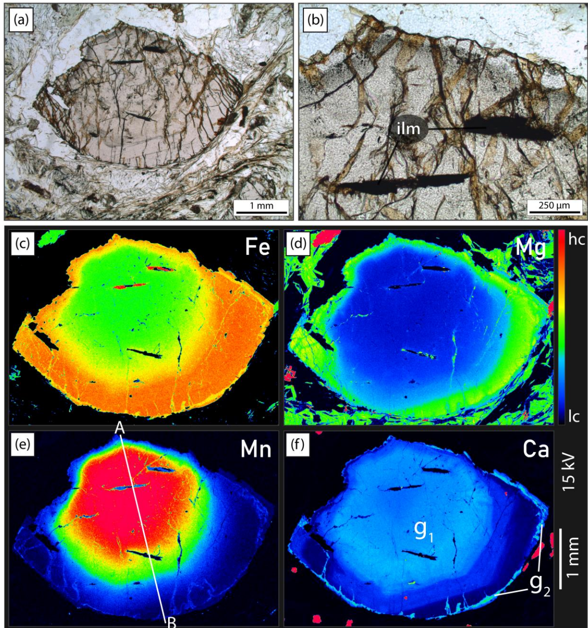
Figure 8. Thin section photomicrographs (PPL) and X-ray maps of a polycyclic garnet from the garnet micaschist GM13. (a) Photomicrograph of polycyclic garnet wrapped by the main Alpine foliation. Garnet is partially dissolved and displays resorbed edges on one side. (b) Ilmenite included in garnet 1 is partially replaced by fine-grained rutile. Along this resorbed edge, garnet 1 is “cloudy” due to the presence of micro-inclusions of graphite, quartz, muscovite and zircon. (c) Fe X-ray map of the garnet shown in (a, b). Ilmenite inclusions in garnet 1 are only partially preserved (lc = low concentration; hc = high concentration). (d) Mg X-ray map. (e) Mn X-ray map. The A-B trace indicates the position of the compositional profile in Figure 7f. (f) Ca X-ray map showing a sharp chemical discontinuity between two garnet generations. Alpine garnet 2 forms a thin and discontinuous overgrowth over the partially dissolved pre-Alpine garnet 1 .
