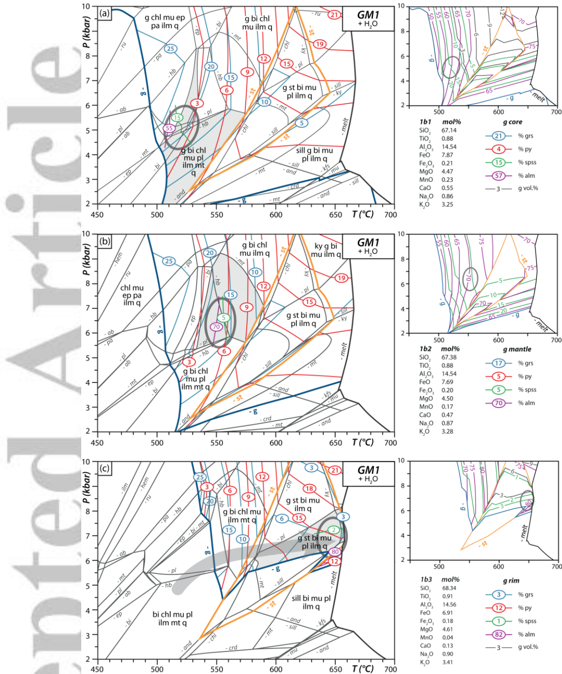
Figure 9. P - T pseudosections calculated for the garnet-staurolite micaschist GM1, considering progressive garnet fractionation. Some fields are not labelled for the sake of clarity; their assemblages can be deduced from assemblages in adjacent fields. The garnet-in, staurolite-in and melt-in lines (wet solidus) are highlighted with thick blue, orange and black lines, respectively. Grey circles indicate the P - T conditions at the three stages of garnet growth. (a) Pseudosection calculated for the bulk composition 1b1 (obtained by XRF) and used for constraining the P - T conditions of equilibration of garnet core. Garnet isomodes are shown in the small plot on the right-hand side. (b) Pseudosection calculated for the bulk composition 1b2 (after garnet core fractionation) and used for constraining the P - T conditions of equilibration of garnet mantle. (c) Pseudosection calculated for the bulk composition 1b3 (after garnet core and mantle fractionation) and used for constraining the P - T conditions of equilibration of garnet rim. The grey arrow indicates the P - T evolution as inferred from the three pseudosections.
