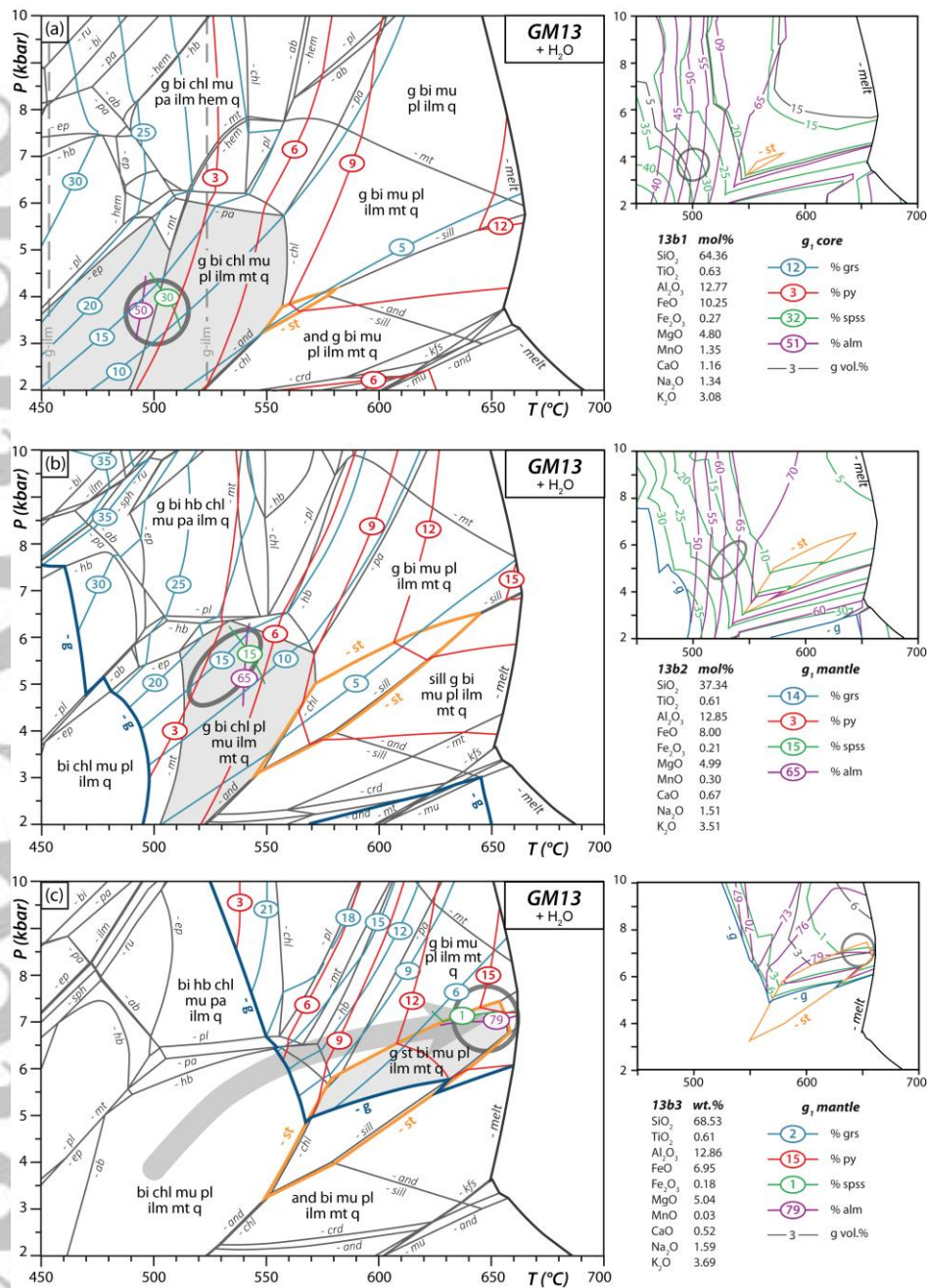
Figure 10. P – T pseudosections calculated for the garnet micaschist GM13, considering progressive garnet fractionation. Some fields are not labelled for the sake of clarity; their assemblages can be deduced from assemblages in adjacent fields. The garnet-in, staurolite-in and melt-in lines (wet solidus) are highlighted with thick blue, orange and black lines, respectively. Garnet composition is used to constrain the P – T conditions (indicated by a grey circle) at the three stages of garnet growth. (a) Pseudosection calculated for the local bulk composition 13b1 (obtained by area scan method) and used for constraining the P – T conditions of equilibration of garnet 1 core. Garnet isomodes are shown in the small plot on the right-hand side. (b) Pseudosection calculated for the bulk composition 13b2 (after garnet 1 core fractionation) and used for constraining the P – T conditions of equilibration of garnet 1 mantle. (c) Pseudosection calculated for the bulk composition 13b3 (after garnet 1 core and mantle fractionation) and used for constraining the P – T conditions of equilibration of garnet 1 rim. The grey arrow indicates the P – T evolution as inferred from the three pseudosections.
