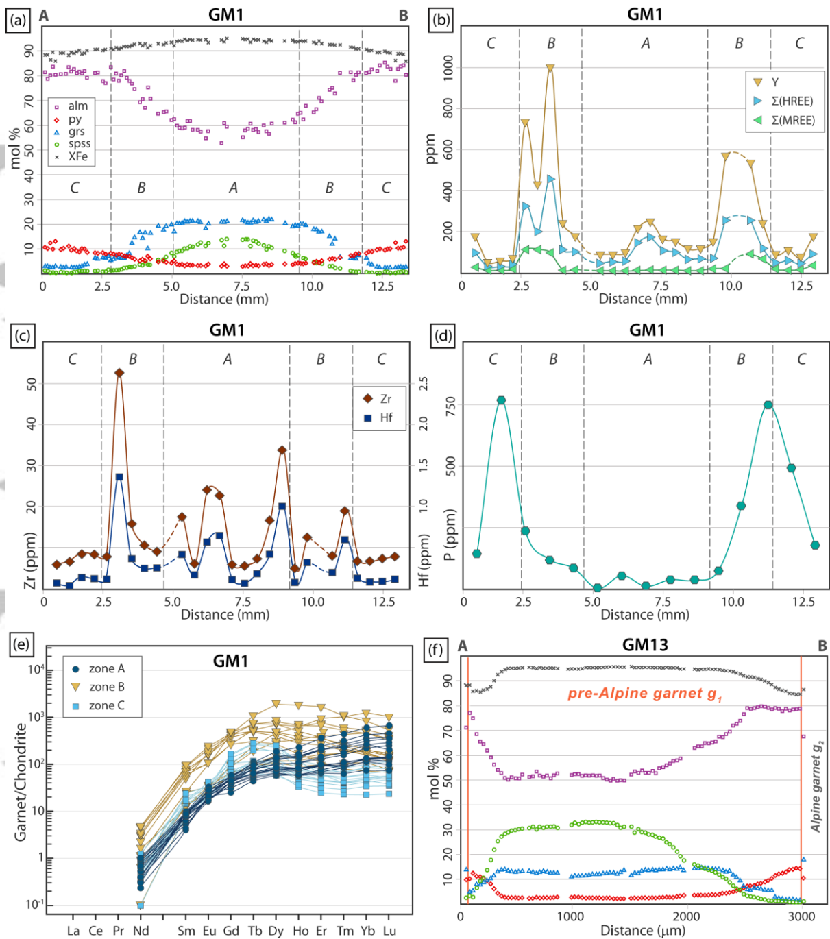
Figure 7. Compositional profile of pre-Alpine garnet from garnet-staurolite micaschist (GM1) for major (a) and trace elements (b, c, d). (b) Compositional profile of Y and sum of HREE and MREE. (c) Compositional profile of Zr and Hf. (d) Compositional profile of P. (e) Chondrite-normalized REE pattern (McDonough & Sun, 1995) for pre-Alpine garnet in sample GM1. (f) Compositional profile of polycyclic garnet from garnet micaschist (GM13) (color coding as in (a)). Vertical orange lines mark the boundaries between the first and second garnet generations. The position of the profiles (a) and (f) is indicated in Figure 6d and Figure 8e, respectively (lines A-B).
