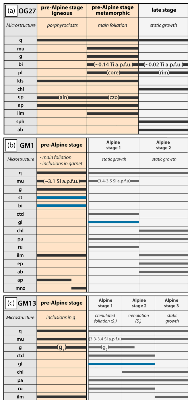
FIGURE 5 Deformation/mineral growth relationships (only observed or pseudomorphed minerals) for the (a) Muret orthogneiss OG27, (b) garnet-staurolite micaschist GM1 and (c) garnet micaschist GM13. The blue line indicates pseudomorphed minerals [Colour figure can be viewed at wileyonlinelibrary.com ] (from 4 to 23 mol.%; Figure 7a). X_{Fe} decreases from 95% to 86% from core to rim (Figure 7a). Distinctive Y oscillations are observed in garnet (Figure 7b). Y is enriched (~250 ppm) in the cores (coreward of zone A), decreases
