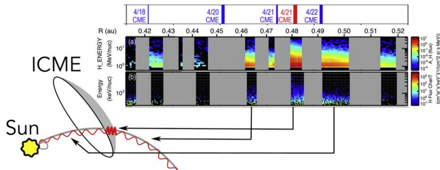
Figure 10. Schematic of the ICME, which drives a compression region (shown by gray region) ahead of the ICME. We show the fluxes observed by IS⊙IS before, during, and after the ICME passage, and indicate where relative to the ICME these populations are observed.
