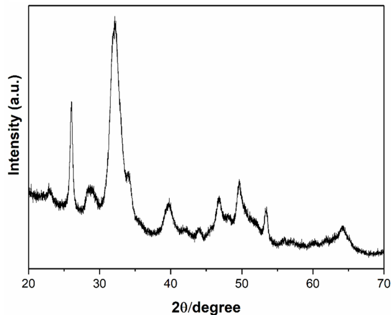
Figure 3. XRD patterns of obtained NBrHAp composite powders.
