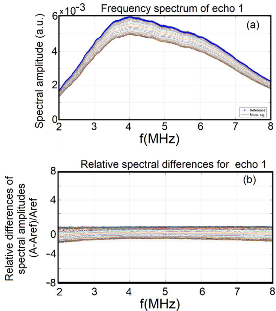
Figure 2. Each recorded signal processed and the frequency spectra (a), and the relative difference of spectral amplitudes during the experiment (b), of NBrHAp suspension.
