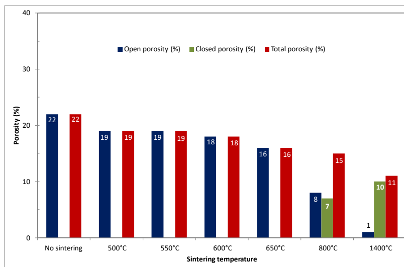
Figure 13. Evolution of the porosity of the Cr pellet with the sintering temperature.
