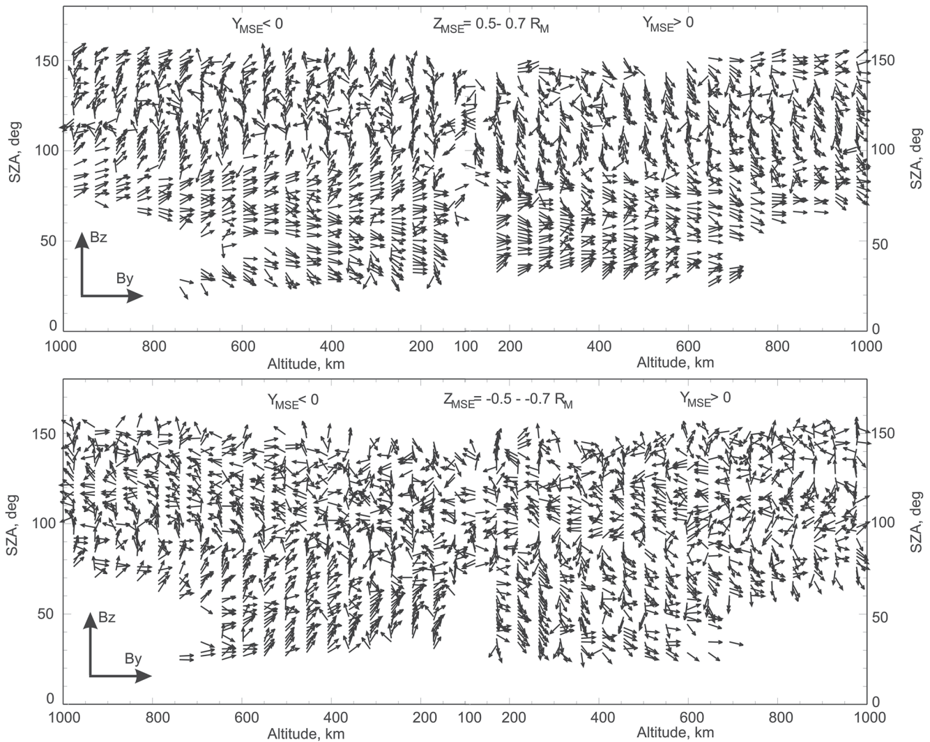
Figure 12. B_z projections of the unit vectors of the magnetic field at Z_{MSE} = 0.5-0.7R_M and Z_{MSE} = -0.5--0.7R_M plotted in the variables altitude and SZA (November 2014–May 2018).
