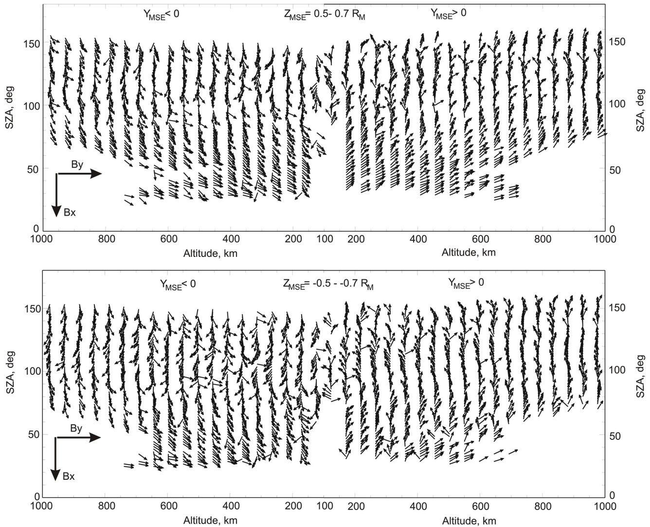
Figure 4. B_{xy} projections of the unit vectors of the magnetic field at Z_{MSE} = 0.5\text{--}0.7R_M and Z_{MSE} = -0.5\text{--}0.7R_M plotted in the variables altitude and SZA (November 2014–August 2017).
