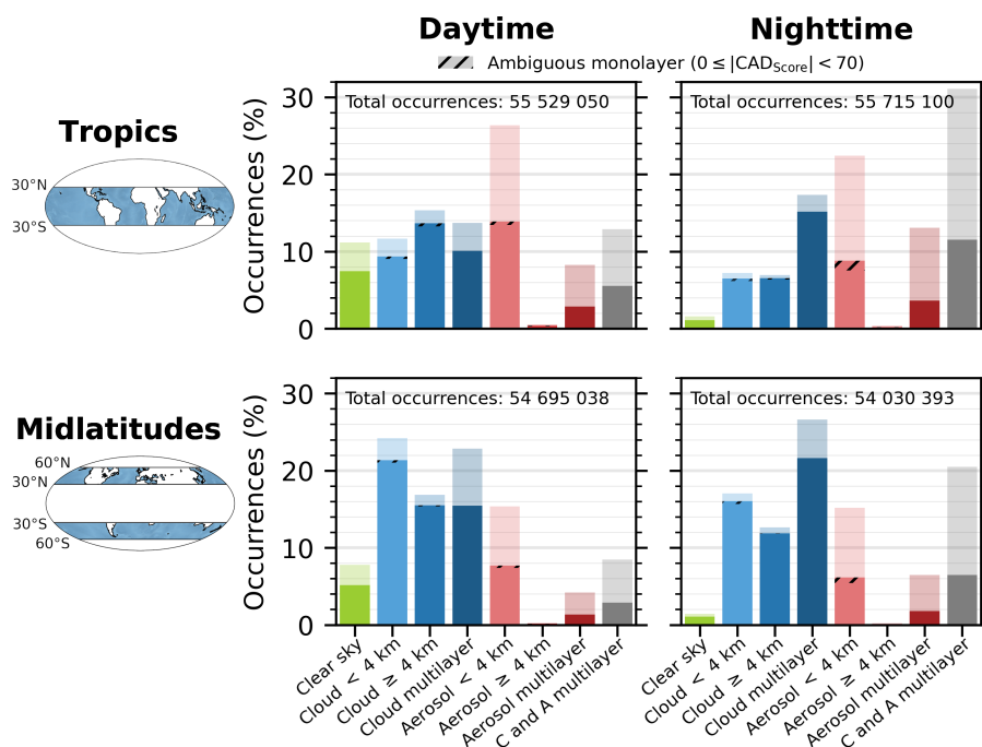
Figure 1. Occurrence of the 5-km atmospheric column types derived from the CALIOP L2 5 km Merged Layer Data Product V4 over ocean during the 2008–2019 period in the tropics [30° S–30° N] (top row) and the midlatitudes [30°–60°] (bottom row) during daytime (left column) and nighttime (right column). The solid bars show the occurrence frequencies of 5-km atmospheric columns in which no clouds were detected at single-shot resolution. The transparent bars show the total occurrence frequencies, i.e., including those columns in which single-shot clouds were detected. For cloud and aerosol monolayer columns (second, third, fifth, and sixth bars), the hatched region of the solid bars shows the CALIPSO V4 CAD ambiguous classification fraction. Layers detected at 80-km-horizontal averaging are not considered in the calculation of occurrence frequencies. Occurrence frequencies for multilayer columns are shown for reference but are not included in this study. Columns containing a monolayer with special CAD score value are not shown here.
