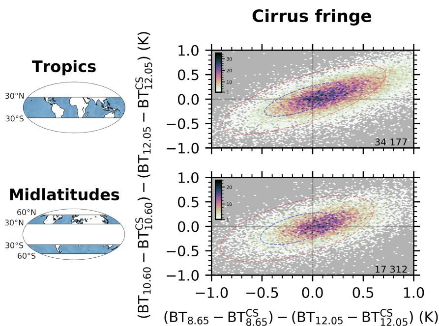
Figure 17. As Fig. 5 but for cirrus fringes with V4 special CAD score of 106, i.e., layers detected as aerosols by the V4 CAD algorithm first and then topped to clouds by the V4 "cirrus fringe amelioration" algorithm (Liu et al., 2019). They mainly are very thin layer (95 % with \tau < 0.2 ) and at high altitude (97 % with z_{\text{top}} > 8 km in the tropics and 22 % with 4 \text{ km} < z_{\text{top}} < 8 km and 78 % with z_{\text{top}} > 8 km in the midlatitudes).
