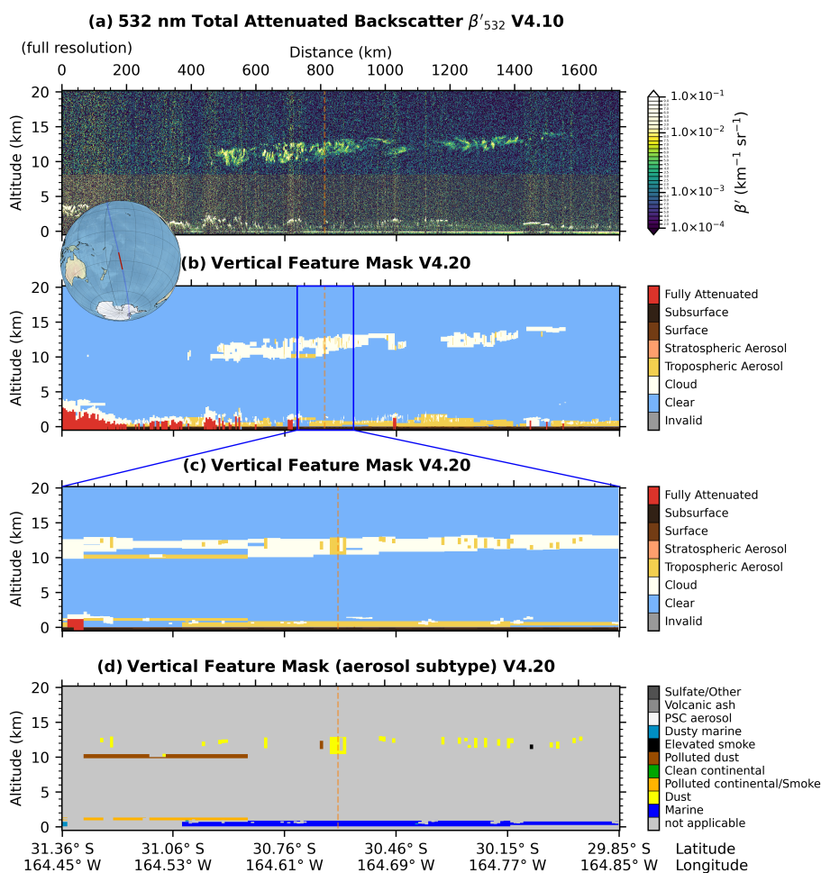
Figure 18. Misclassified dust monolayer by V4 CAD algorithm ( \text{CAD}_{\text{score},V4} = -36 ) identified as cloud by IIR observation ( \text{CAD}_{\text{score},IIR} = 99 ). The misclassified aerosol layer is located between 10.5 and 12.9 km altitude in the 5-km atmospheric column (5-km index #1541) indicated by a dashed line. CALIOP daytime observations on 1 March 2018, 1:01:13–1:05:25 UTC, over the South Pacific: (a) 532 nm total attenuated backscatter V4.10, (b) vertical feature mask V4.20, (c) vertical feature mask zoom around the atmospheric column of interest, and (d) aerosol subtyping. The marine aerosol layer in the planetary boundary layer is detected with 80-km-horizontal averaging and does not affect the IIR observation.
