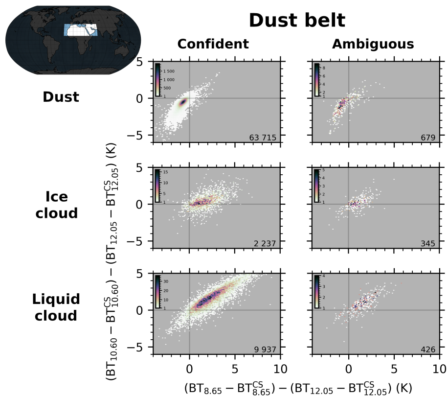
Figure 9. As Fig. 2 for dust, ice cloud, and liquid cloud detected in the dust belt region ( 10^{\circ} N– 38^{\circ} N and 25^{\circ} W– 65^{\circ} E) with 4 < z_{top} < 8 km and 0.2 < \tau < 3 .
