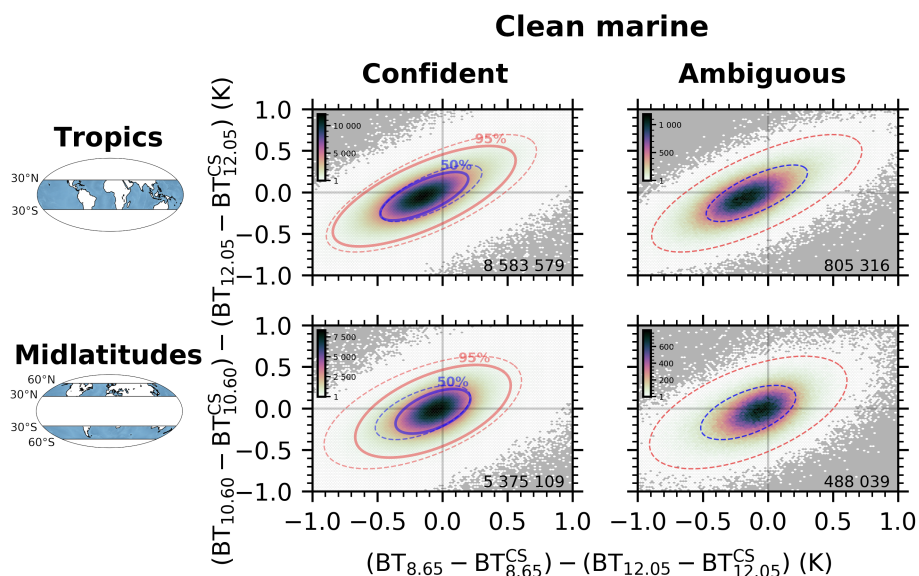
Figure 7. As Fig. 5 for clean marine monolayer observations with \tau < 0.2 and z_{top} < 4 km (99 % of all clean marine observations). The red and blue solid ellipses represent the 95 % and 50 % confidence intervals of the 2-D gaussian PDF estimated from the confident observations of this specific z_{top}-\tau grid and used in the IIR CAD score definition (Eq. (1)).
