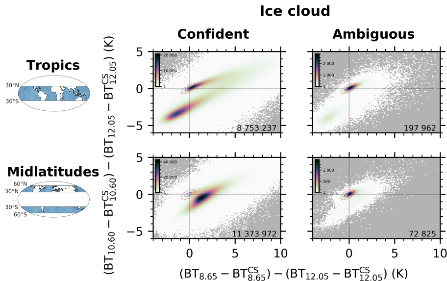
Figure 5. As Fig. 2 for ice cloud monolayer observations considered as confident ( 70 \leq |CAD_{score,V4}| \leq 100 ) (left column) and ambiguous ( 0 \leq |CAD_{score,V4}| < 70 ) (right column) by the CALIPSO V4 algorithm. The red and blue dashed ellipses represent the observed 95 % and 50 % confidence intervals of IIR clear-sky observations (see Fig. 2).
