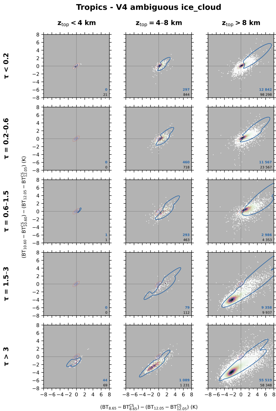
Figure 15. IIR signature of the V4 ambiguous ( 0 \leq |CAD_{score,V4}| < 70 ) ice cloud observations for the 2008–2019 period in the tropics. IIR signature inside the blue contour ( |CAD_{score,IIR}| \geq 70 ) are confidently classified as cloud by the IIR CAD algorithm. At the bottom-right corner of each subplot are indicated the total number of V4 ambiguous ice cloud observations (black) and those that are confidently classified as cloud by IIR (blue).
