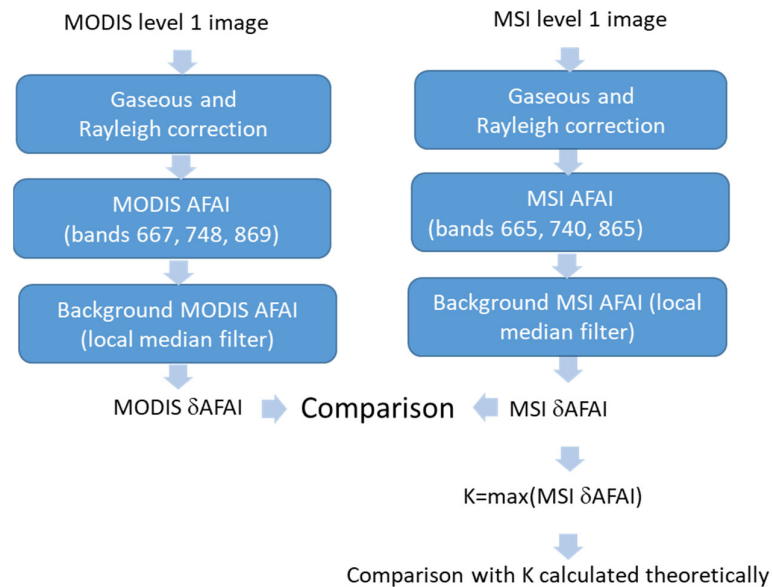
Figure 5. Flowchart of the overall methodology used to compare MODIS/ \delta AFAI and MSI/ \delta AFAI and to empirically estimate the slope K of the linear relationship between \delta AFAI and the fractional coverage (FC).
