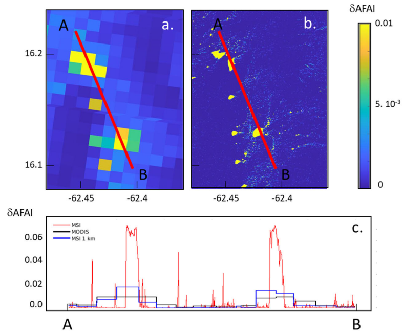
Figure 3. (a) MODIS/ \delta AFAI/(a) and (b) MSI/ \delta AFAI on 21 June 2018 for the same site (site #1), and (c) \delta AFAI values along the AB transect where the red line corresponds to MSI-20 m, the black line to MODIS 1 km, and the blue line to MSI-1 km.
