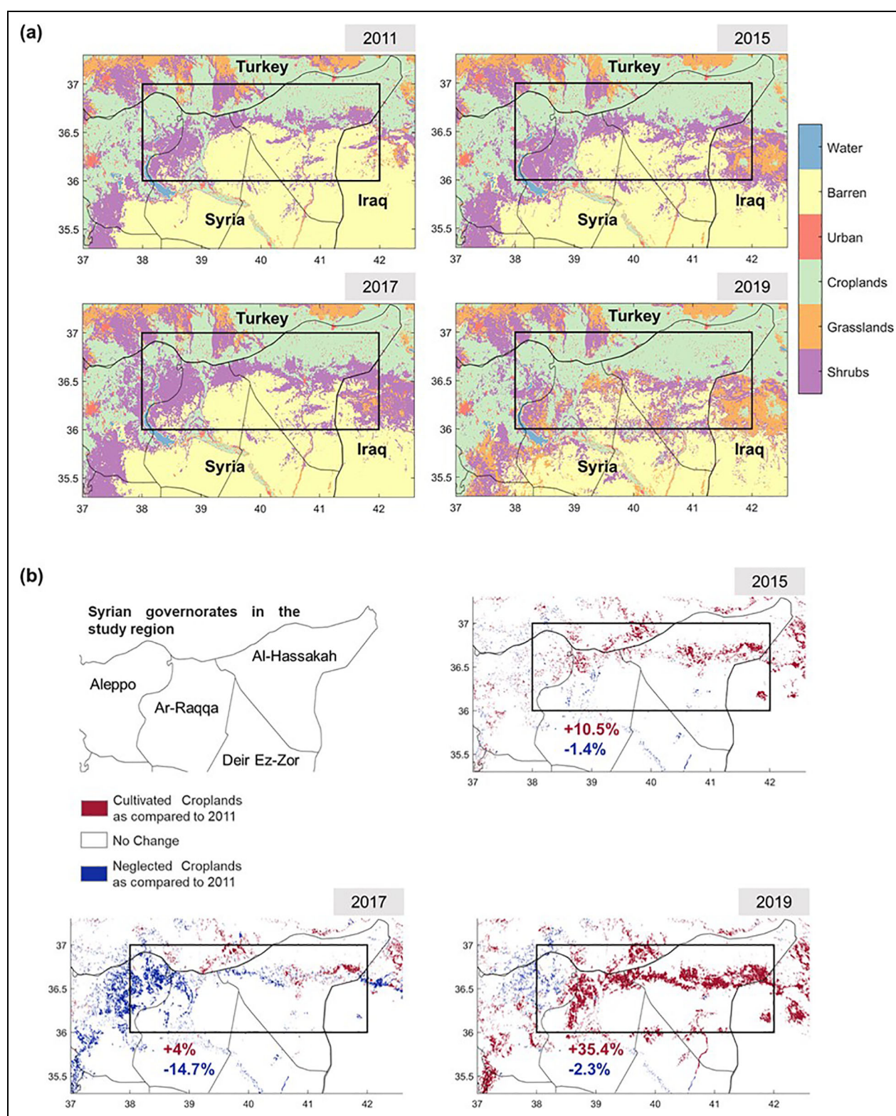
Figure 3. (a) Yearly distribution of MODIS land cover over northeast Syria (500 × 500 m²). The region of study is shown in the black rectangle for the years 2011 (start of the war), 2015 (Islamic State in control of most of the region), 2017 (intense clashes between Islamic State, Kurdish forces and other groups), and 2019 (better security conditions). Only relevant land cover classifications are shown here; (b) Yearly evolution (neglected or cultivated) of MODIS croplands as compared to croplands for the year 2011. “Cultivated Croplands” (red pixels)/“Neglected Croplands” (blue pixels) represent croplands that were cultivated/abandoned during the designated year in comparison to 2011. The evolution (expansion/abandonment) of croplands (indicated in red/blue) is calculated in comparison to 2011 and for pixels located in Syria only. DOI: https://doi.org/10.1525/elementa.2021.000041.f3
