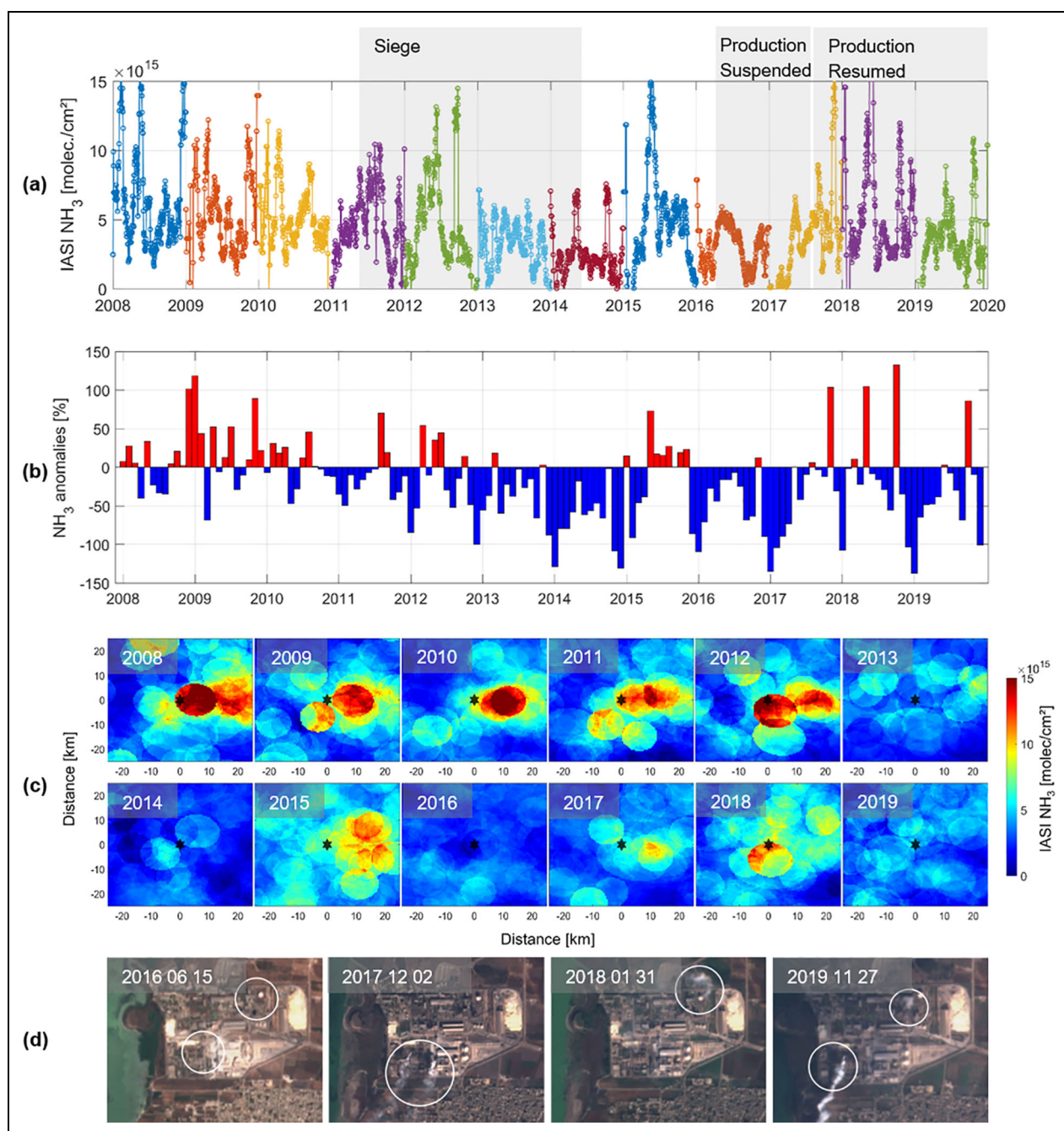
Figure 2. (a) 20-day running mean of IASI daily total columns of ammonia (molec/cm 2 ) averaged over the fertilizers industry ( 0.5 \times 0.5^\circ grid box centered on the factory). (b) Monthly percentage anomalies of IASI total columns of ammonia over the GFC, compared with [2008–2012] monthly averages. (c) Oversampled yearly spatial average of IASI NH 3 total columns (molec/cm 2 ) around the fertilizers industry (indicated with a black star). (d) Sentinel 2 L1C satellite images of the fertilizers company on days of suspension of activities (2016), and resume of production (2017, 2018 and end of 2019). DOI: https://doi.org/10.1525/elementa.2021.000041.f2
