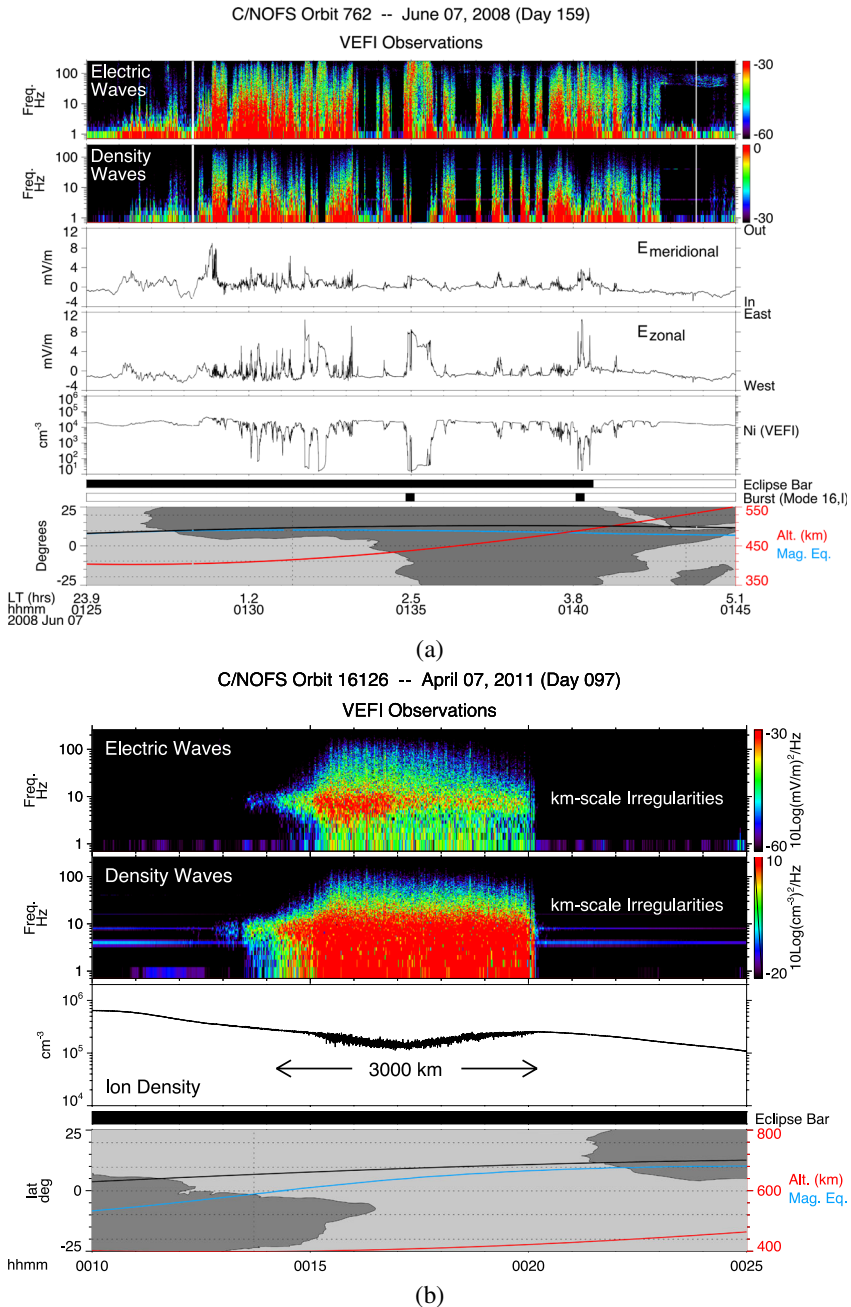
Fig. 72 (a) Plasma density from the VEFI Langmuir probe (lowest data panel) above which is plotted the DC electric field, showing the strong correspondence of the zonal electric fields and the plasma density depletions. The upper two panels shown the spectrograms of the electric and density data sampled at 512 s/sec. The lowest panels include the eclipse bar, burst bar, and map showing the C/NOFS location. (b) Plasma density from the VEFI Langmuir probe (lowest data panel) showing a wide swath ( \sim 3000 km horizontal distance) of km scale waves appearing near 10 Hz in the density and electric field spectrograms (upper two panels). The lowest panels include the eclipse bar and map showing the C/NOFS location
