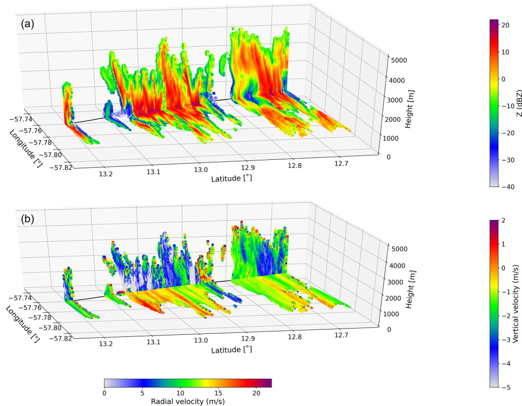
Figure 15. (a) Reflectivity corrected for attenuation (dBZ) and (b) Doppler velocity (vertical component V_z and radial component V_x ; \text{m s}^{-1} ) from the vertically pointing RASTA radar and from the horizontally pointing BASTA radar displayed as a function of height (for RASTA) or horizontal range (for BASTA), along a subcloud-layer leg during RF17 (from 09:06:09 to 09:20:03 UTC on 11 February 2020).
