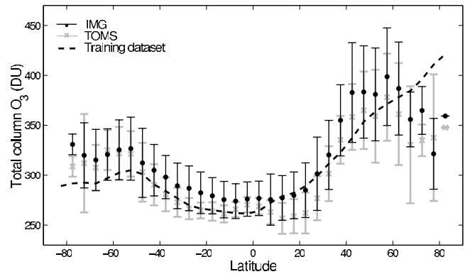
Figure 4. Total O 3 derived from co-located IMG/ADEOS and TOMS/ADEOS measurements, and from the O 3 training set, zonally averaged over the four periods analyzed (with associated standard deviations).
