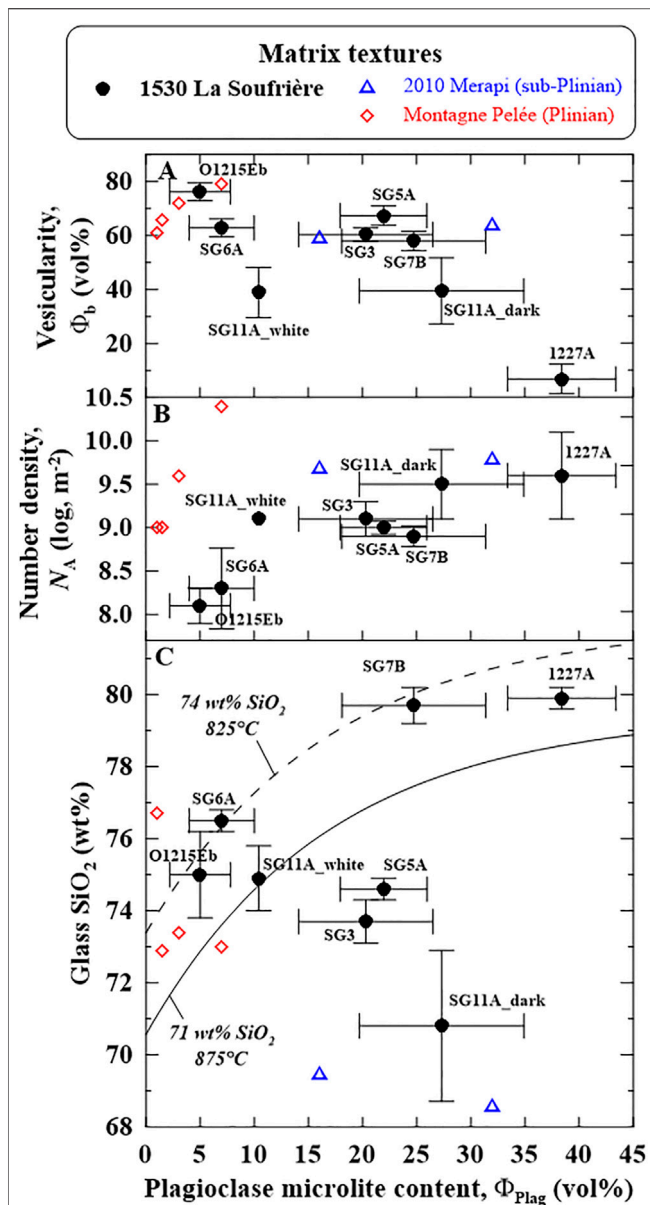
FIGURE 3 | Matrix textures defined as the content of the plagioclase microlites versus (A) vesicularity, (B) number density of plagioclase microlites, and (C) SiO 2 content of the residual glasses; sample numbers as in Table 1; the curves represent equilibrium crystallization starting from melts with 71 and 74 wt% SiO 2 (plain and dashed lines, respectively), as calculated from combining Eq. 3 with Eq. 4 and Eq. 6 in Supplementary Material. For comparison, the blue triangles represent the November 5, 2010 sub-Plinian event of Merapi, Indonesia (from Preece et al., 2014), and the red diamonds show the P1, P2, P3, and P4 Plinian eruptions of Montagne Pelée, Martinique (Martel and Poussineau, 2007).
