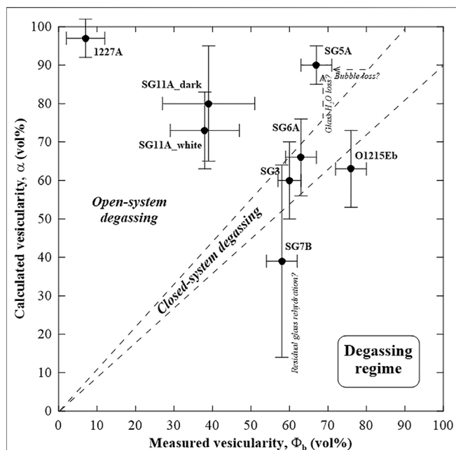
FIGURE 8 | Degassing regime, as defined by the vesicularity measured in the natural samples ( \Phi_b in Table 1) versus the vesicularity calculated after Eq. 1 in Supplementary Material (Jaupart and Allègre, 1991) for a closed-system degassing for which the gas bubbles stay in the magma. The 1:1 line (enlarged to 10% uncertainty) delimits a closed-system degassing, for which measured and calculated vesicularities compare, to an open-system degassing regime, for which bubbles are lost (outgassing) so that the measured vesicularities are lower than calculated for a closed-system degassing. The error bars give the statistical errors on the vesicularity measurements (X-axis) and the variability of the calculations resulting from the range of residual glass H_2O contents (Y-axis), as given in Table 1.
