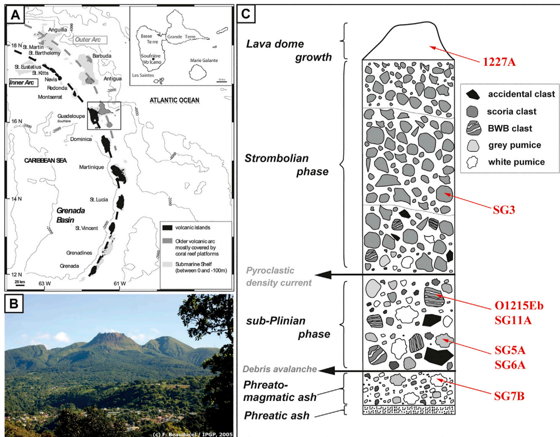
FIGURE 1 | (A) Location map of the Lesser Antilles, Guadeloupe archipelago, and La Soufrière volcanic complex, after Boudon et al. (2008), (B) Photo of La Soufrière present dome and (C) Typical stratigraphy section of the AD 1530 eruption, combining the sequence deposits at the sites of the Carbet Springs and Gallion River (Boudon et al., 2008), showing the origin of the studied samples (from Boudon et al., 2008; Pichavant et al., 2018).
