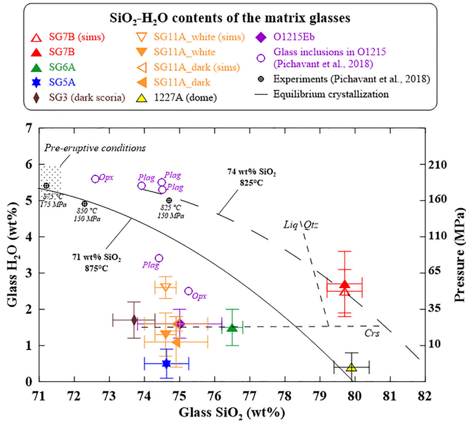
FIGURE 6 | \text{H}_2\text{O} versus \text{SiO}_2 content of the matrix glasses. The \text{H}_2\text{O} contents are determined by the by-difference method using the electron microprobe, except where "(sims)" is mentioned which refers to \text{H}_2\text{O} determination by ion probe (as given in Table 1 ). Pressures on the right Y-axis are \text{H}_2\text{O} solubility pressures calculated after Newman and Lowenstern (2002). The purple open circles are the glass inclusion data given in Pichavant et al. (2018). The crossed circles are experiments from Pichavant et al. (2018) and the colored box gives the experimentally-determined pre-eruptive conditions. The curves show the trends for equilibrium crystallization starting from a 71 wt% \text{SiO}_2 melt (plain curve; after Eq. 4 in Supplementary Material ) and from a 74 wt% \text{SiO}_2 melt (dashed curve; after Eq. 6 in Supplementary Material ). The dashed lines show the silica polymorph boundaries in rhyolitic melts as defined in Martel et al. (2021).
