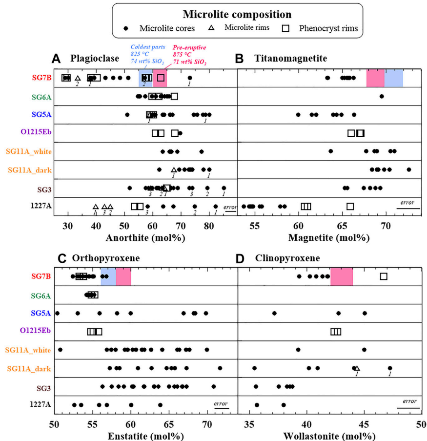
FIGURE 4 | Compositions of the microlites of (A) plagioclase in An mol%, (B) titanomagnetite in Mt mol%, (C) orthopyroxene in En mol%, and (D) clinopyroxene in Wo mol%. The red box gives the pre-eruptive compositions at 175 MPa and 875°C determined experimentally for the phreatomagmatic SG7B pumice sample by Pichavant et al. (2018) and the blue box represents those assumed for coldest (~825°C) parts of the reservoir.
