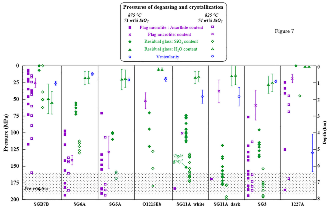
FIGURE 7 | Equilibrium pressures of crystallization and degassing calculated from the anorthite content of the plagioclase microlites (Eq. 2 at 875°C and Eq. 5 at 825°C in Supplementary Material ), the content of plagioclase microlite (Eq. 3 in Supplementary Material ), the \text{SiO}_2 content of the residual glasses (Eq. 4 at 875°C and Eq. 6 at 825°C in Supplementary Material ), the \text{H}_2\text{O} content of the residual glass (from Newman and Lowenstern, 2002), and sample vesicularity (Eq. 1 in Supplementary Material ). All pressures calculated at more than 200 MPa are not shown. The dashed box gives the range of pre-eruptive pressure determined by Pichavant et al. (2018).
