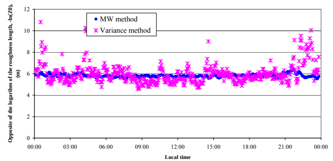
Fig. 8b. Roughness length. Comparison between the statistical method MW and the variance method (Plot RT, 25 July 1997).
