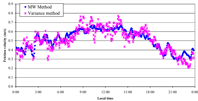
Fig. 7b. Friction velocity. Comparison between the statistical method MW and the variance method (Plot RT, 25 July 1997).
