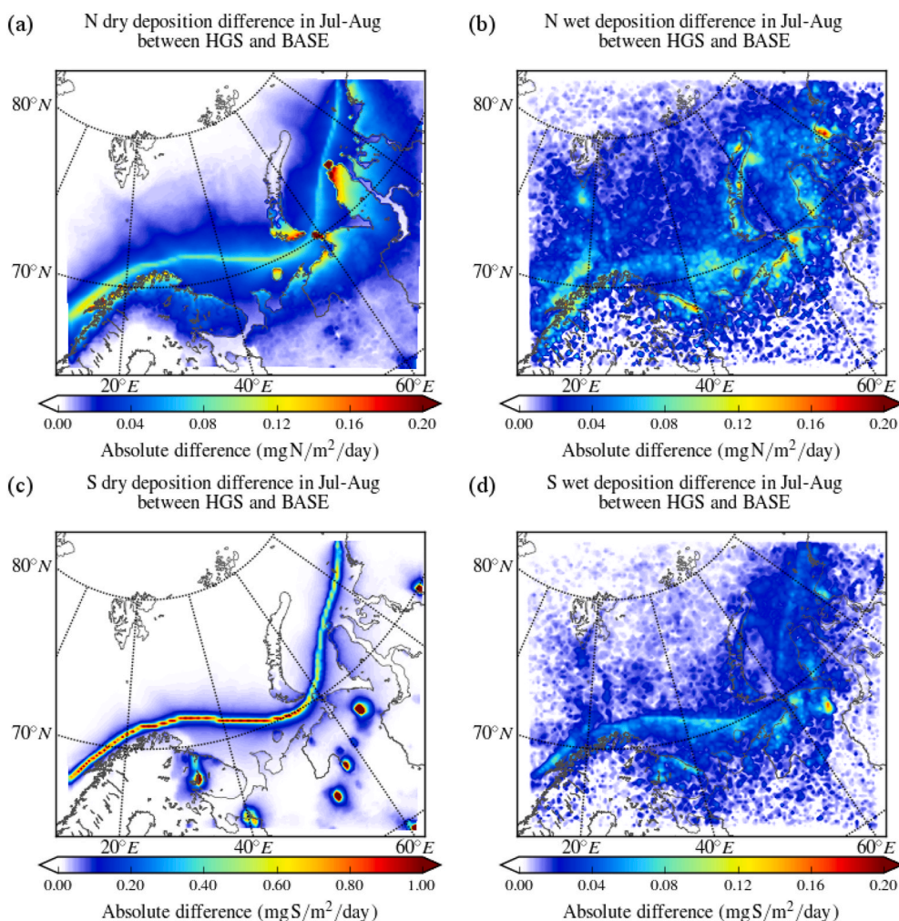
Fig. 6. Absolute differences in monthly mean dry (a,c) and wet (b,d) deposition fluxes of total nitrogen (in mgN/m 2 /day) (a,b) and total sulphur (in mgS/m 2 /day) (c, d) between the HGS scenario and the BASE run.
