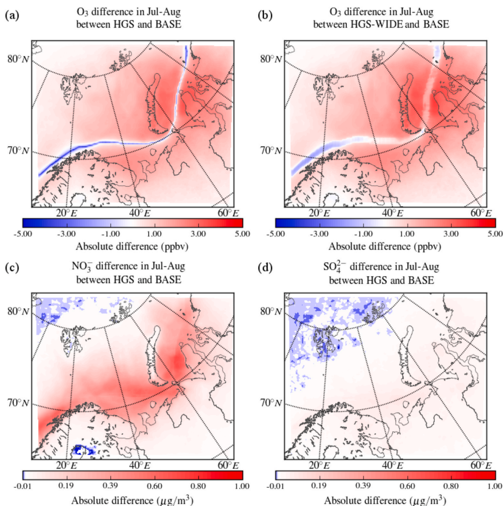
Fig. 4. Absolute differences in monthly mean surface O_3 mixing ratios (in ppbv) (a), nitrate aerosol concentrations (in \mu\text{g m}^{-3} ) (c) and sulphate aerosol concentrations (in \mu\text{g m}^{-3} ) (d) between the HGS scenario and the BASE run. Panel (b) shows the absolute difference in monthly mean surface O_3 mixing ratios between the HGS-WIDE scenario and the BASE run.
