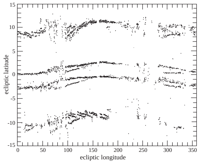
Fig. 53. Observed ecliptic latitude of the peak brightness of the asteroidal bands as function of the ecliptic longitude of the viewing direction (basically as function of the orbital motion of the earth). The expected sinusoidal variation is evident but distorted, since the elongation of the viewing direction was modulated on an approximately monthly timescale, and because observations both east and west of the sun were contained in the data set. Taken from Reach (1992)
