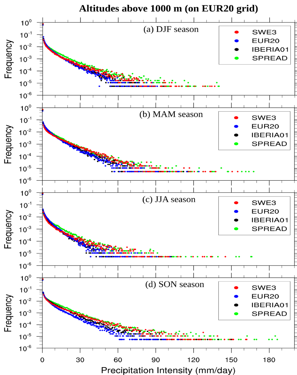
Fig. 13 Probability density function (PDF) of daily mean precipitation (frequency versus intensity) over the Iberian Peninsula (IP, over the area above the altitudes of 1000 m of the SPREAD observation) from the EUR20 (blue), and SWE3 (red), IBERIA01 (black), SPREAD (green) regridded on the EUR20 grid for a DJF, b MAM, c JJA, and d SON seasons during 2000–2009. Units are in mm day -1
