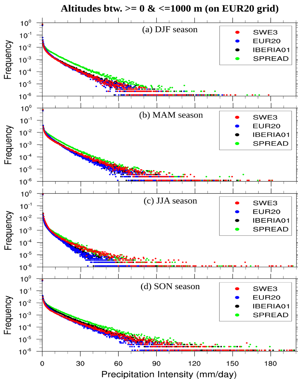
Fig. 12 Probability density function (PDF) of daily mean precipitation (frequency versus intensity) over the Iberian Peninsula (IP, over the area between the altitudes of >=0 and <=1000 m of the SPREAD observation) from the EUR20 (blue), and SWE3 (red), IBERIA01 (black), SPREAD (green) regridded on the EUR20 grid for a DJF, b MAM, c JJA, and d SON seasons during 2000–2009. Units are in \text{mm day}^{-1}
