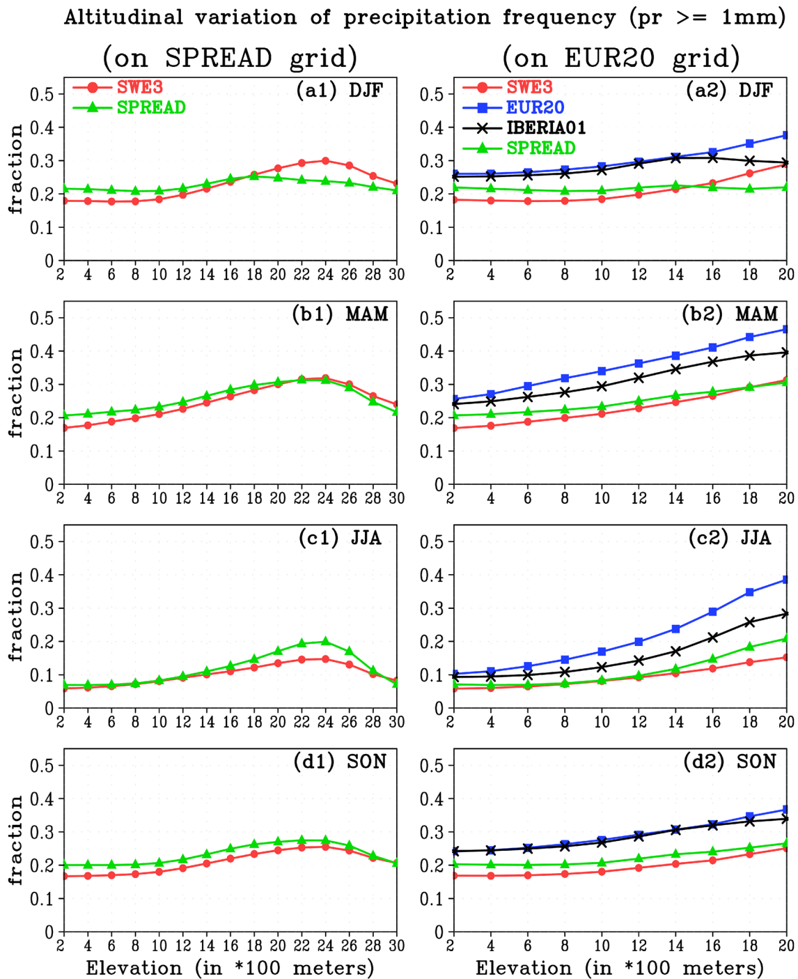
Fig. 8 Altitudinal distribution of precipitation frequency (days where precipitation >= 1 mm) from the SWE3 (red), EUR20 (blue), IBERIA01 (black), and SPREAD (green) over the Iberian Peninsula (IP, over the area of SPREAD observation) on the SPREAD & EUR20
