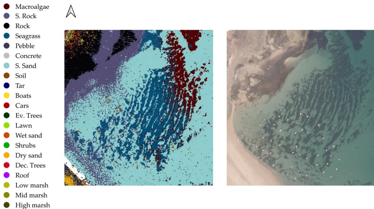
Figure 12. Seagrass meadow classification: Extract of the projected 3D map of the habitats obtained with the predictions of a random forest classifier on green spectral features, infrared intensities, and elevation values, and extract of an orthoimage of the same area. The orthoimage was captured in 2014, while lidar data are not contemporaneous as they date from 2019. S. = submerged, Ev. = evergreen, Dec. = deciduous.
