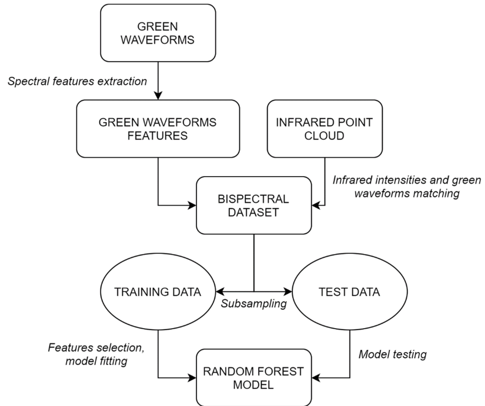
Figure 6. Flowchart of the overall methodology.
