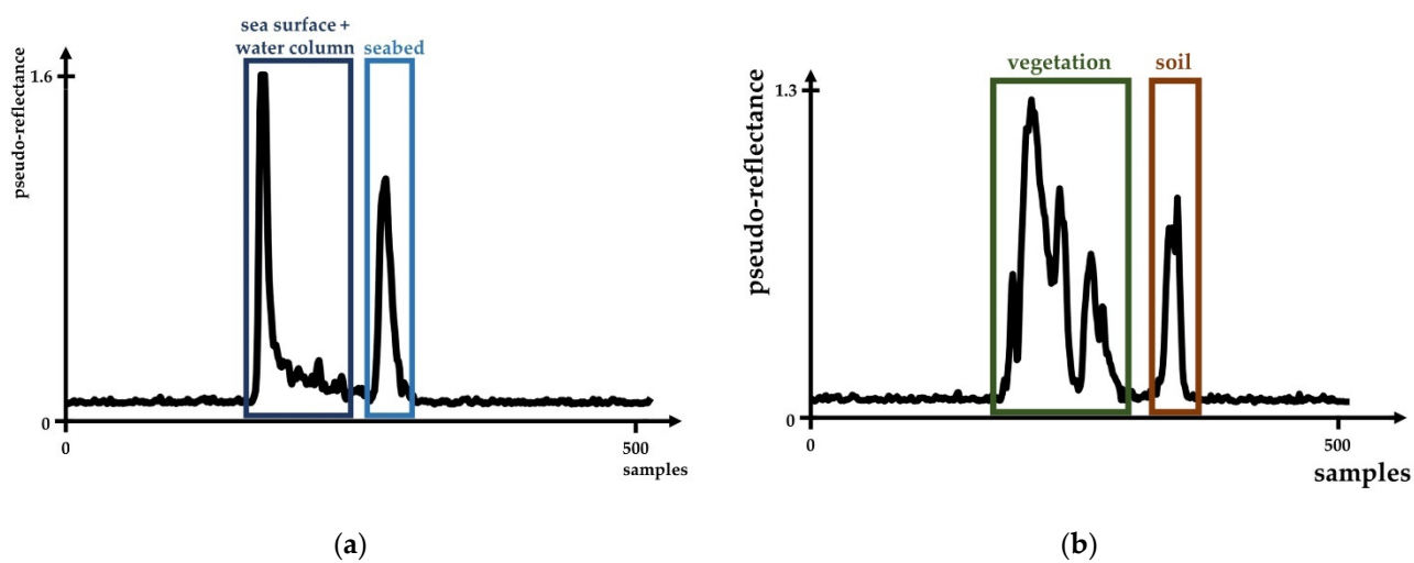
Figure 2. Examples of typical lidar waveforms (for a green laser with a wavelength of 515 nm). (a) Bathymetric waveform acquired in a coastal area; (b) topographic waveform acquired in a vegetated area. A sample corresponds to 556 picoseconds.
